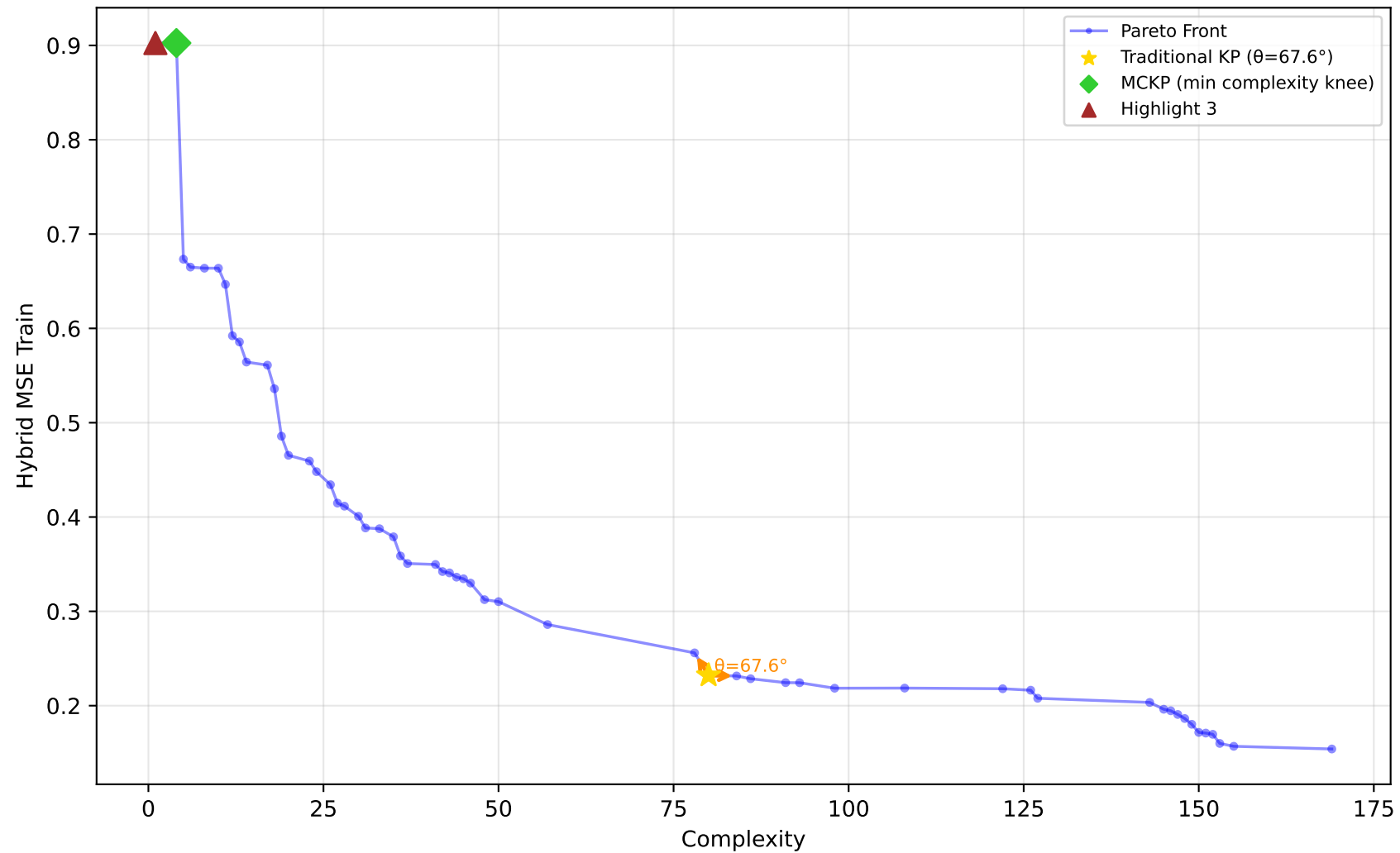
522_pm10 - Run 1 - MVP - Hybrid MSE Train \lambda_1=0.00, \lambda_2=0.90, \lambda_3=0.00 | Difficulty: 1.00 | Method: hmr
