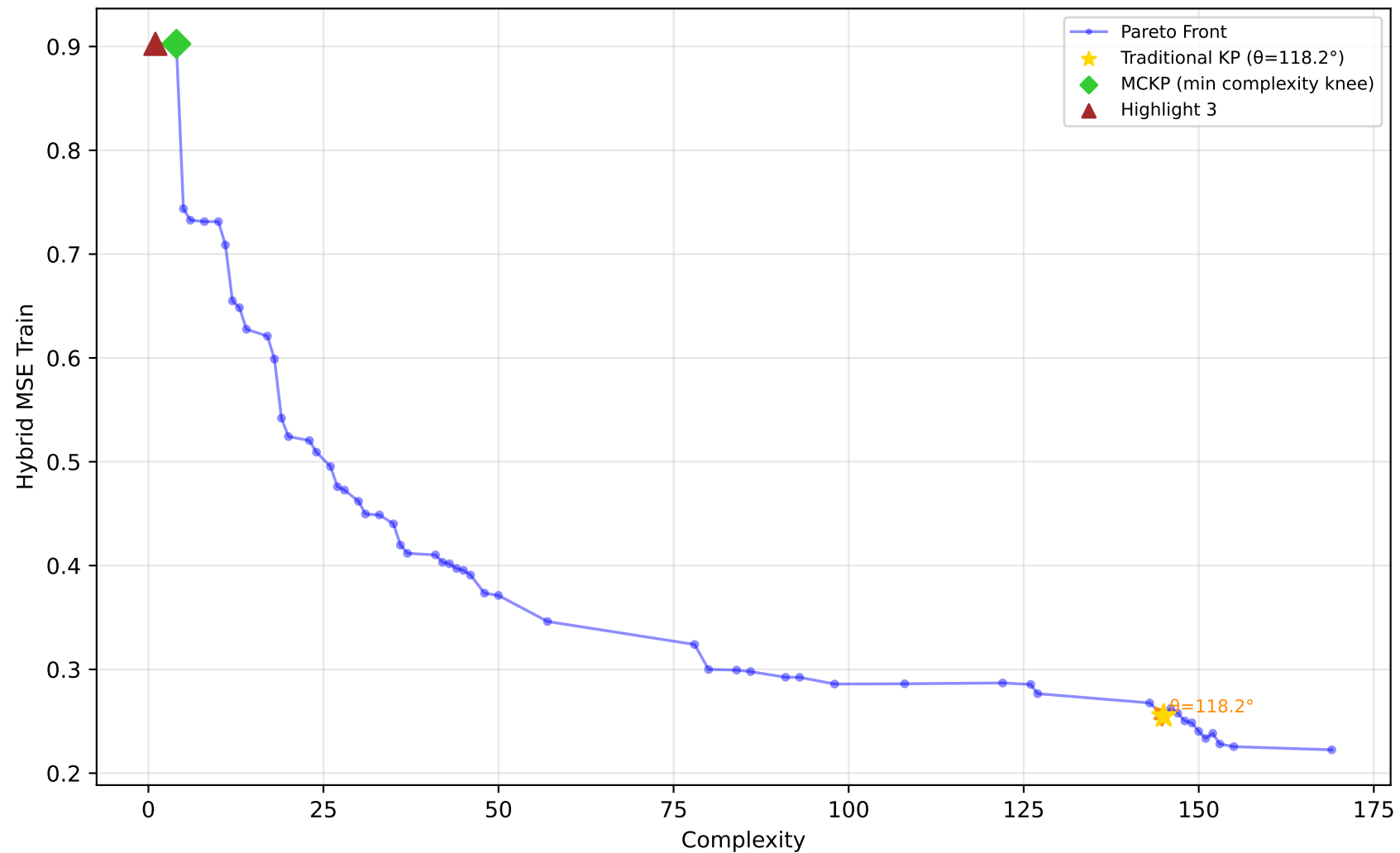
522_pm10 - Run 1 - MVP - Hybrid MSE Train \lambda_1=1.00, \lambda_2=0.00, \lambda_3=0.00 | Difficulty: 1.00 | Method: hmr
