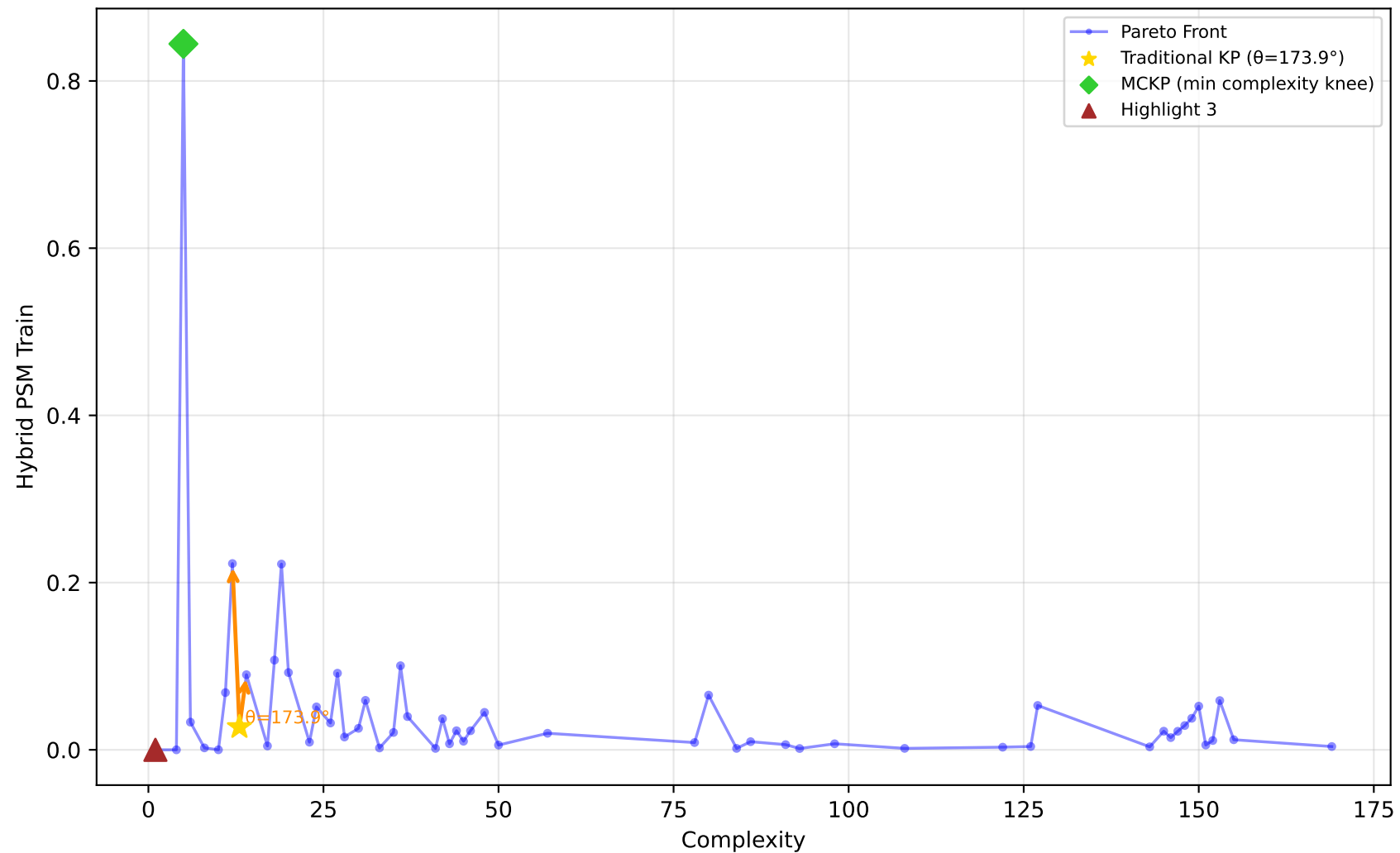
522_pm10 - Run 1 - MVP - Hybrid PSM Train \lambda_1=0.00, \lambda_2=0.90, \lambda_3=0.00 | Difficulty: 1.00 | Method: hmr
