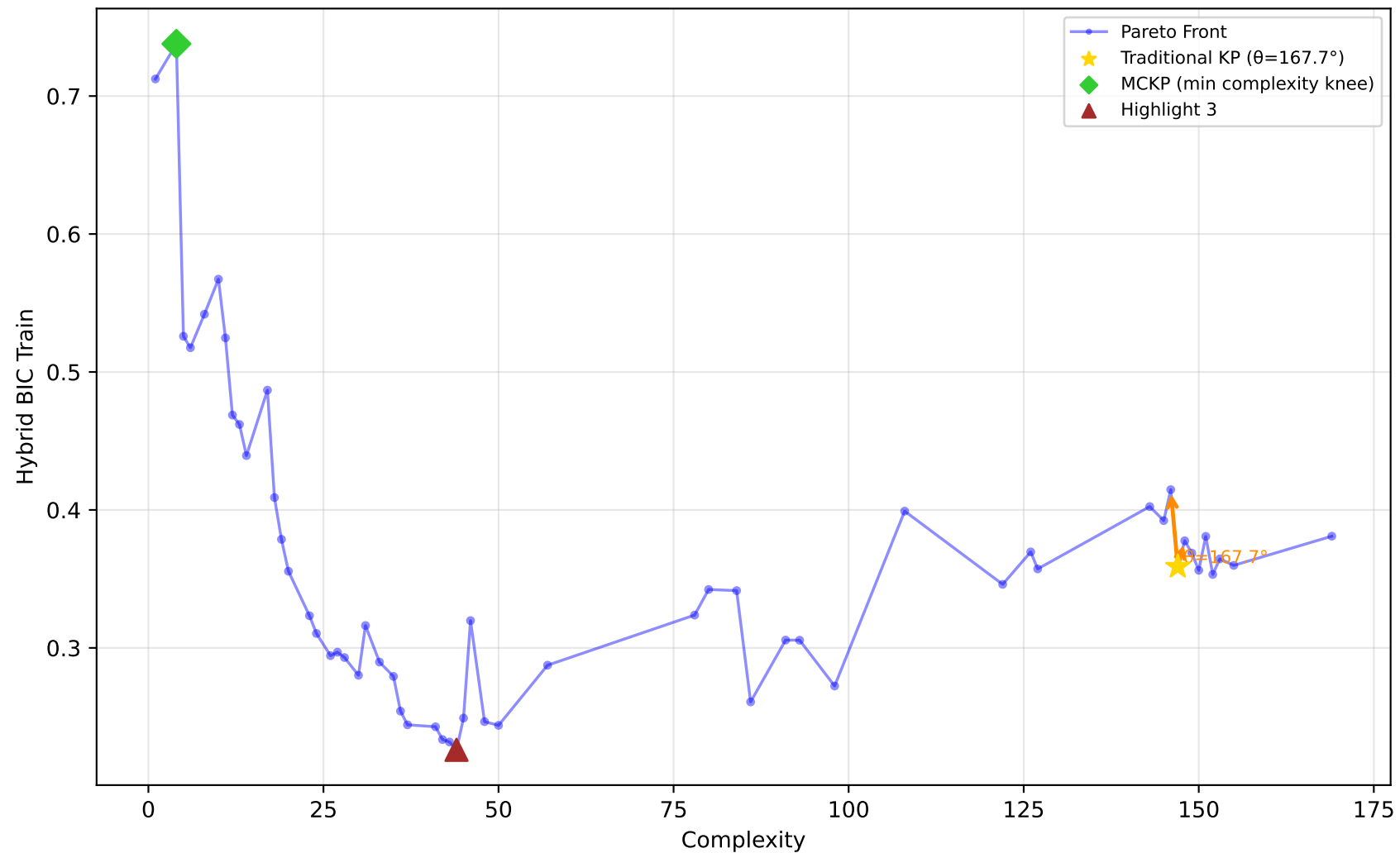
522_pm10 - Run 1 - SVP - Hybrid BIC Train \lambda_1=0.00, \lambda_2=0.10, \lambda_3=0.00 | Difficulty: 1.00 | Method: hmr
