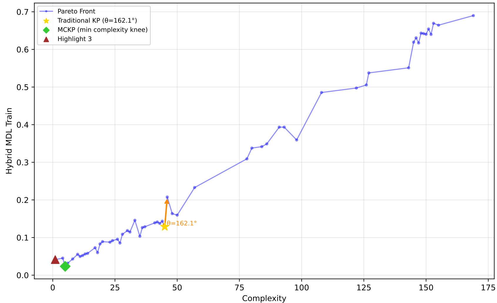
522_pm10 - Run 1 - SVP - Hybrid MDL Train \lambda_1=0.00, \lambda_2=0.10, \lambda_3=0.00 | Difficulty: 1.00 | Method: hmr
