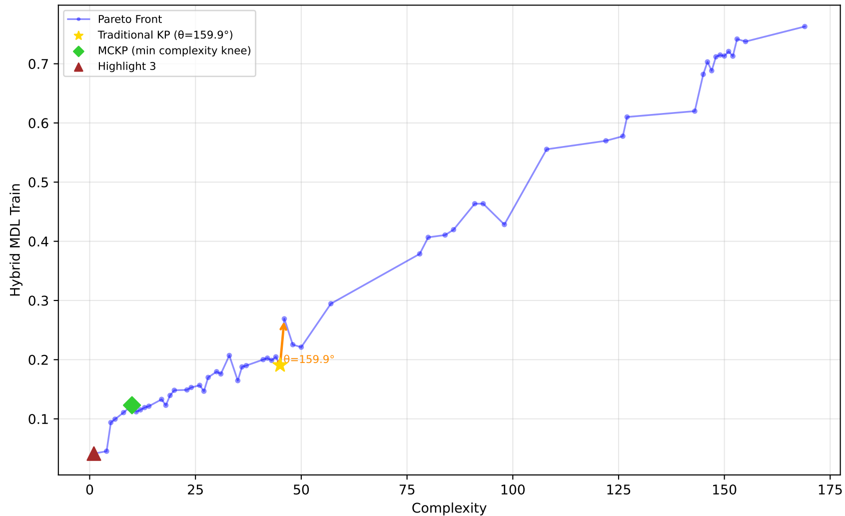
522_pm10 - Run 1 - SVP - Hybrid MDL Train \lambda_1=1.00, \lambda_2=0.00, \lambda_3=0.90 | Difficulty: 1.00 | Method: hmr
