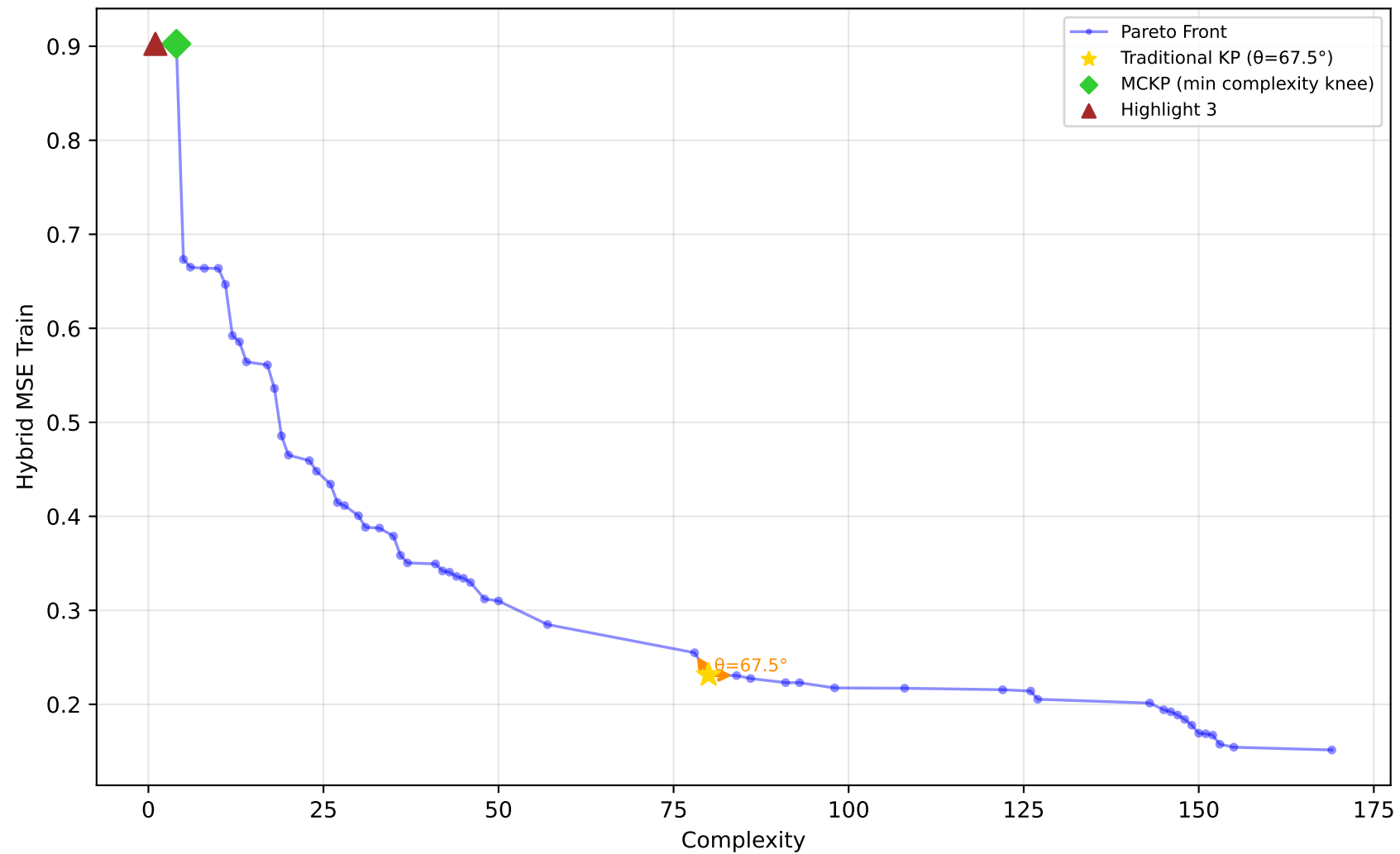
522_pm10 - Run 1 - SVP - Hybrid MSE Train \lambda_1=0.00, \lambda_2=0.10, \lambda_3=0.00 | Difficulty: 1.00 | Method: hmr
