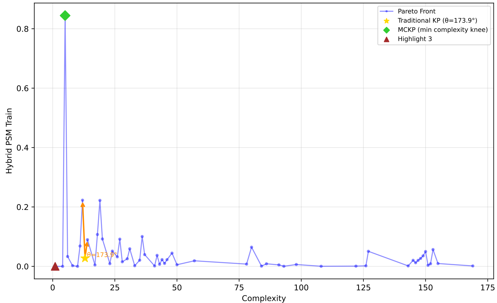
522_pm10 - Run 1 - SVP - Hybrid PSM Train \lambda_1=0.00 , \lambda_2=0.10 , \lambda_3=0.00 | Difficulty: 1.00 | Method: hmr
