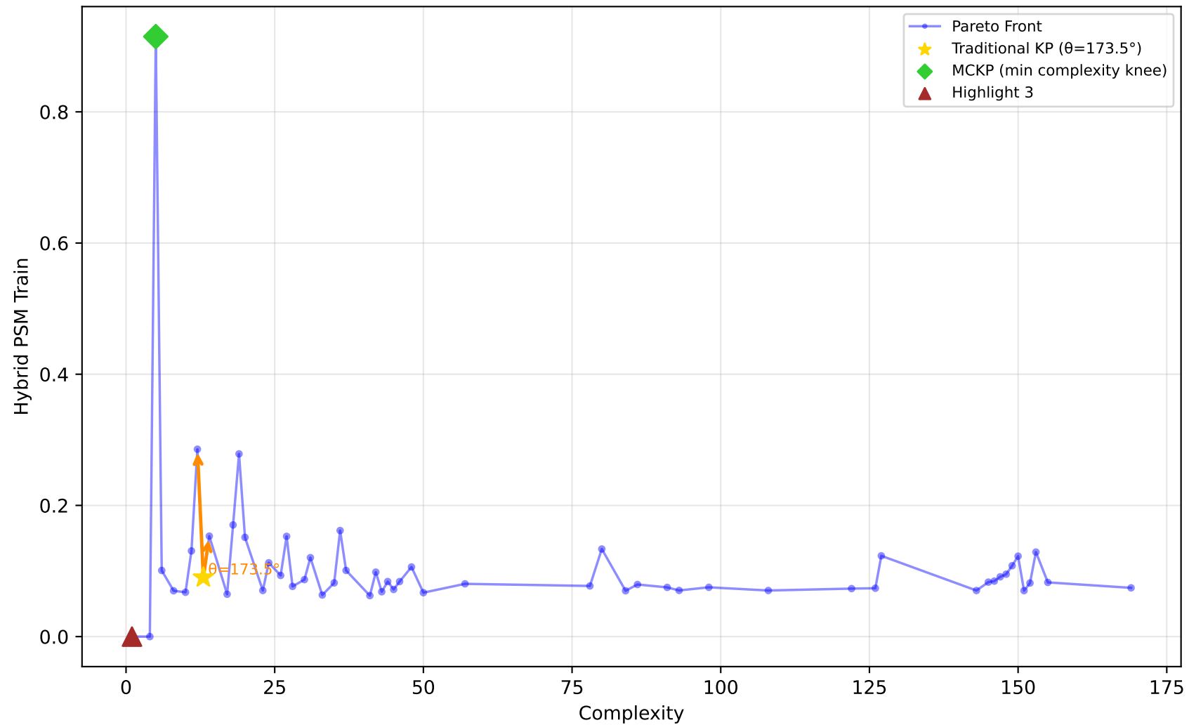
522_pm10 - Run 1 - SVP - Hybrid PSM Train \lambda_1=1.00, \lambda_2=0.00, \lambda_3=0.90 | Difficulty: 1.00 | Method: hmr
