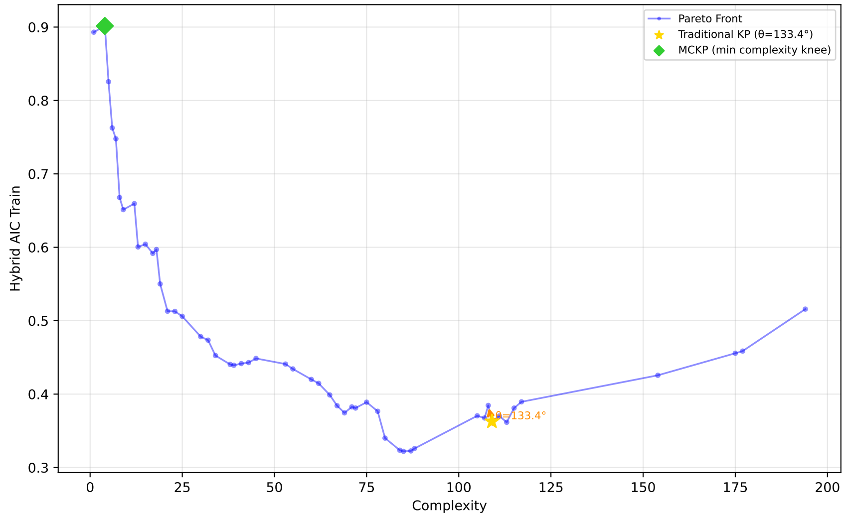
522_pm10 - Run 20 - MVP - Hybrid AIC Train \lambda_1=1.00, \lambda_2=0.00, \lambda_3=0.00 | Difficulty: 1.00 | Method: hmr
