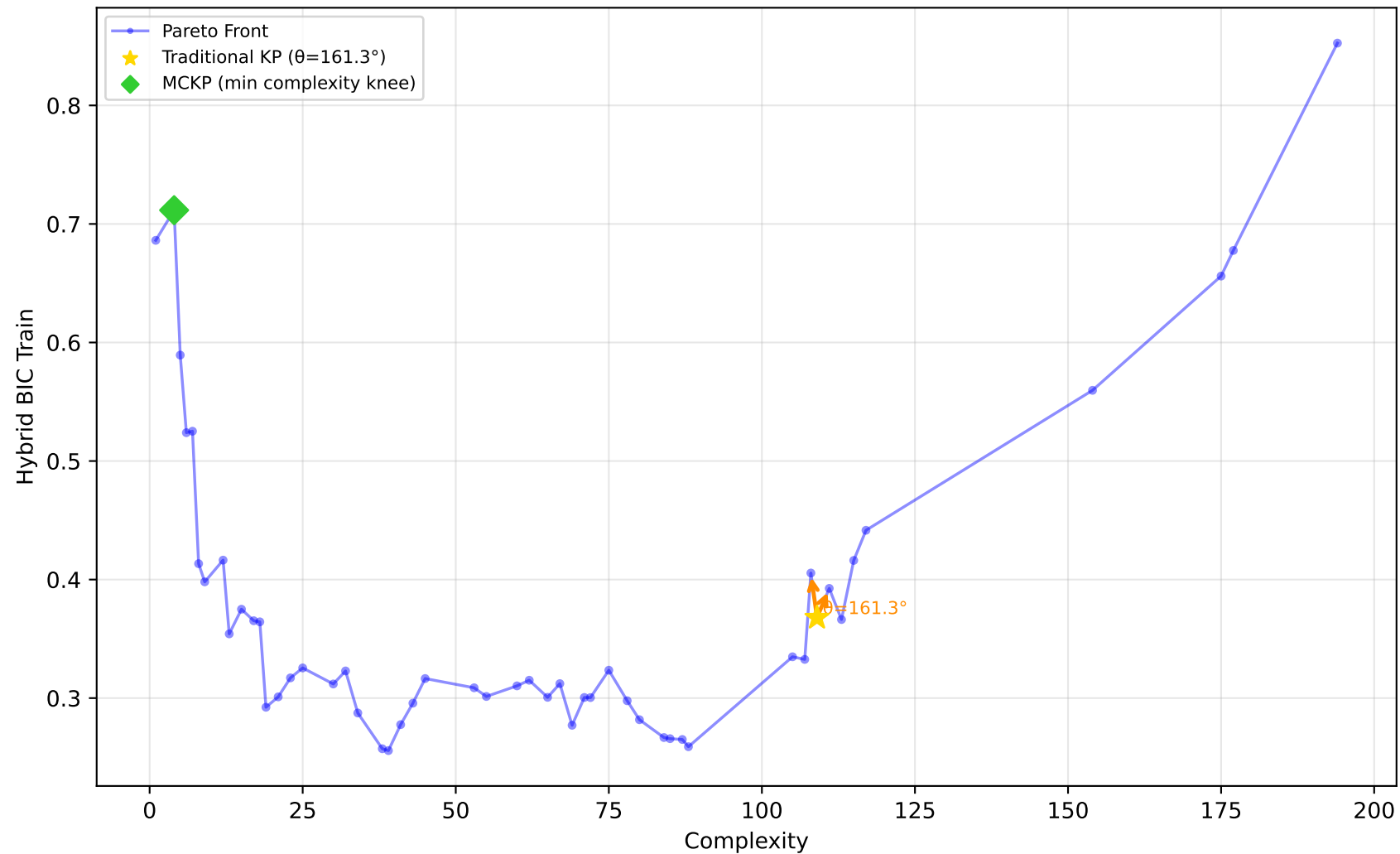
522_pm10 - Run 20 - MVP - Hybrid BIC Train \lambda_1=0.00, \lambda_2=0.90, \lambda_3=0.00 | Difficulty: 1.00 | Method: hmr
