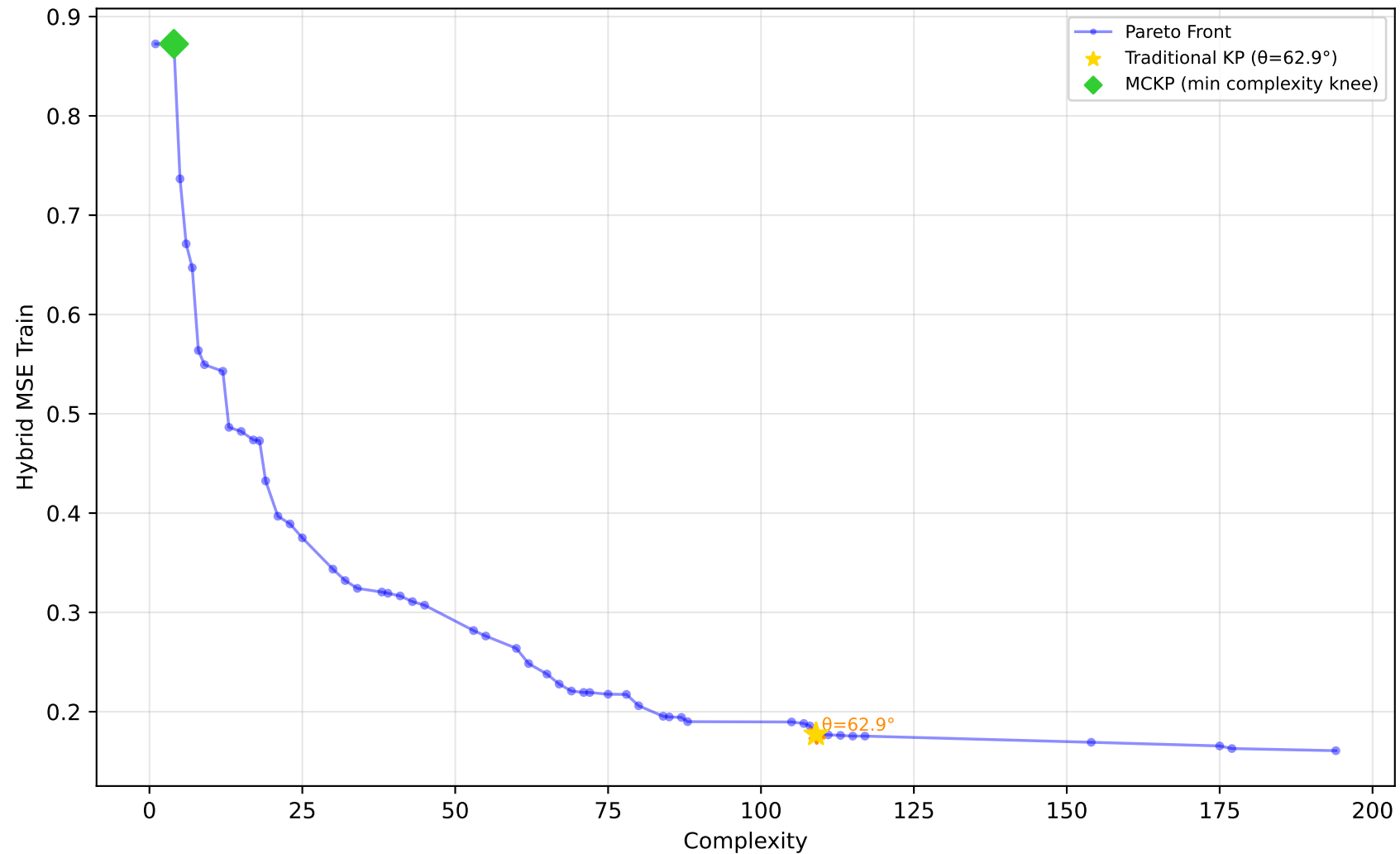
522_pm10 - Run 20 - MVP - Hybrid MSE Train \lambda_1=0.00, \lambda_2=0.90, \lambda_3=0.00 | Difficulty: 1.00 | Method: hmr
