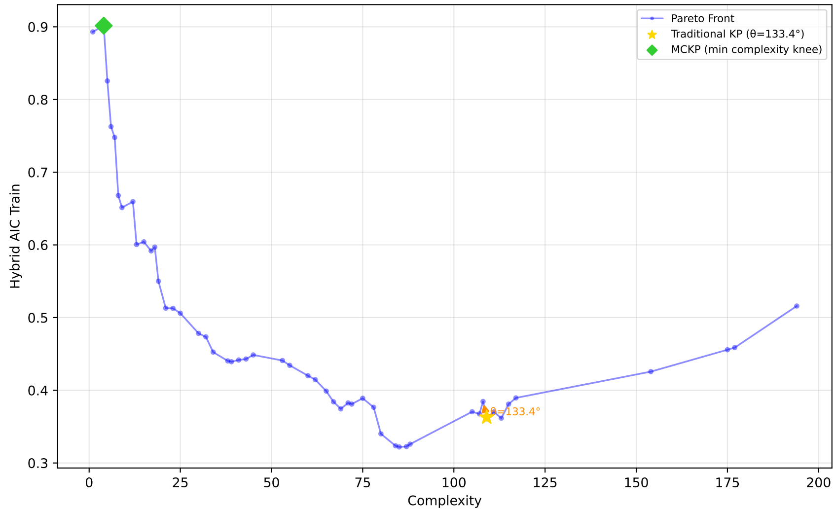
522_pm10 - Run 20 - SVP - Hybrid AIC Train \lambda_1=1.00, \lambda_2=0.00, \lambda_3=0.90 | Difficulty: 1.00 | Method: hmr
