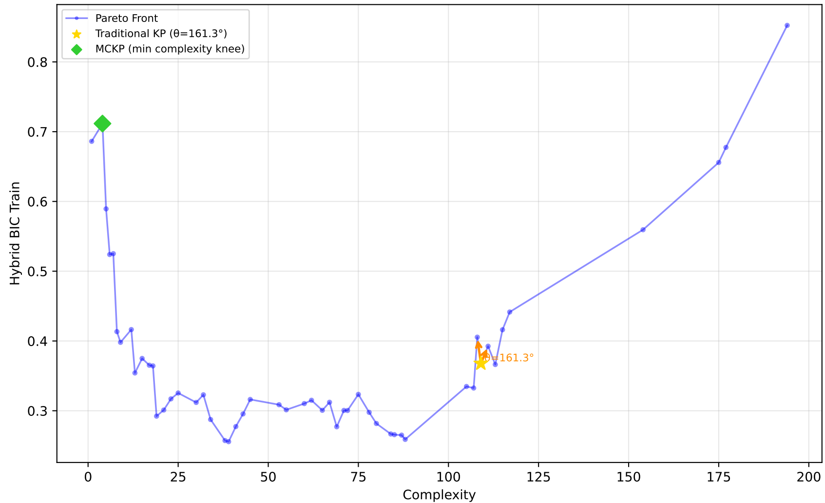
522_pm10 - Run 20 - SVP - Hybrid BIC Train \lambda_1=0.00, \lambda_2=0.10, \lambda_3=0.00 | Difficulty: 1.00 | Method: hmr
