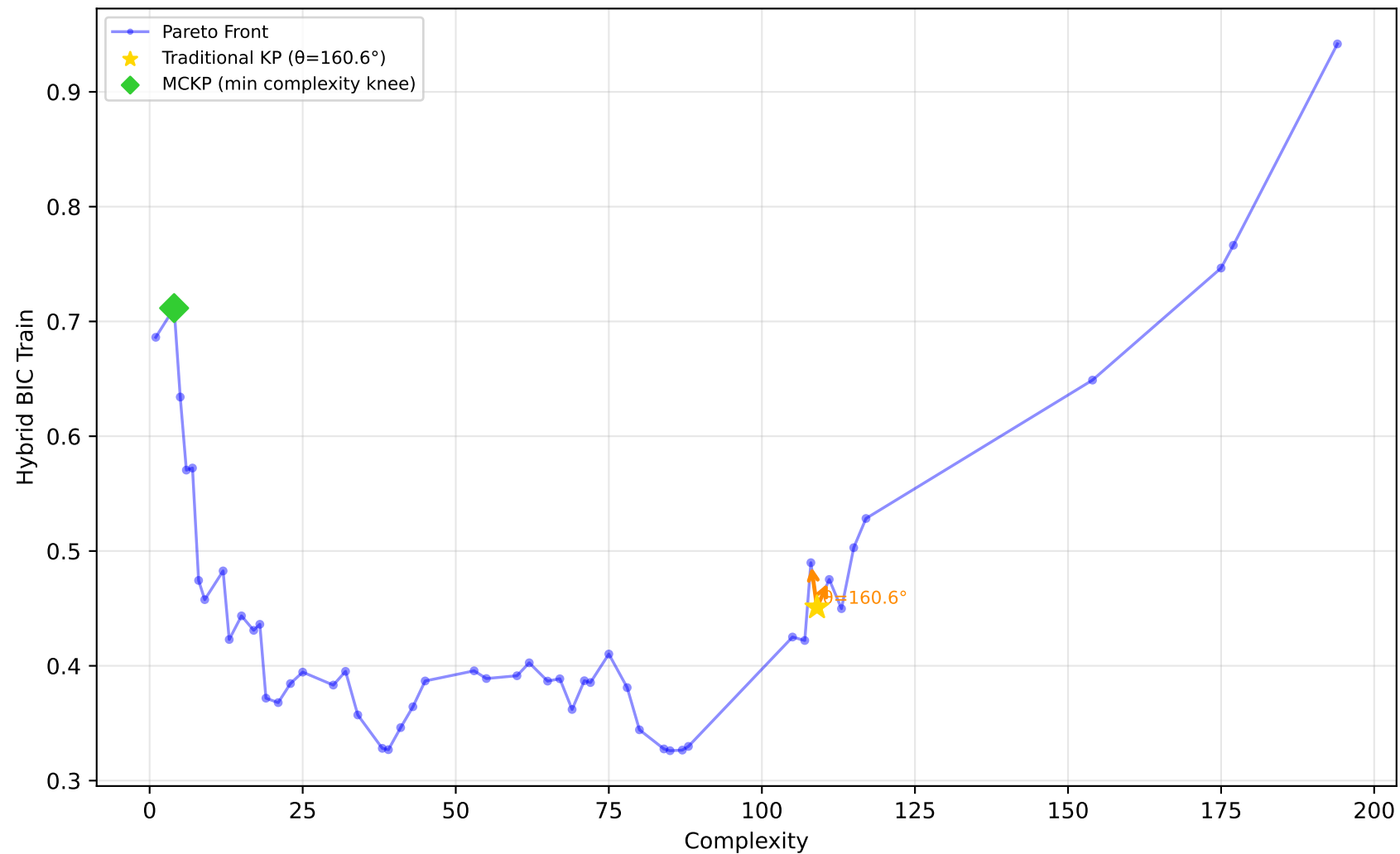
522_pm10 - Run 20 - SVP - Hybrid BIC Train \lambda_1=1.00, \lambda_2=0.00, \lambda_3=0.90 | Difficulty: 1.00 | Method: hmr
