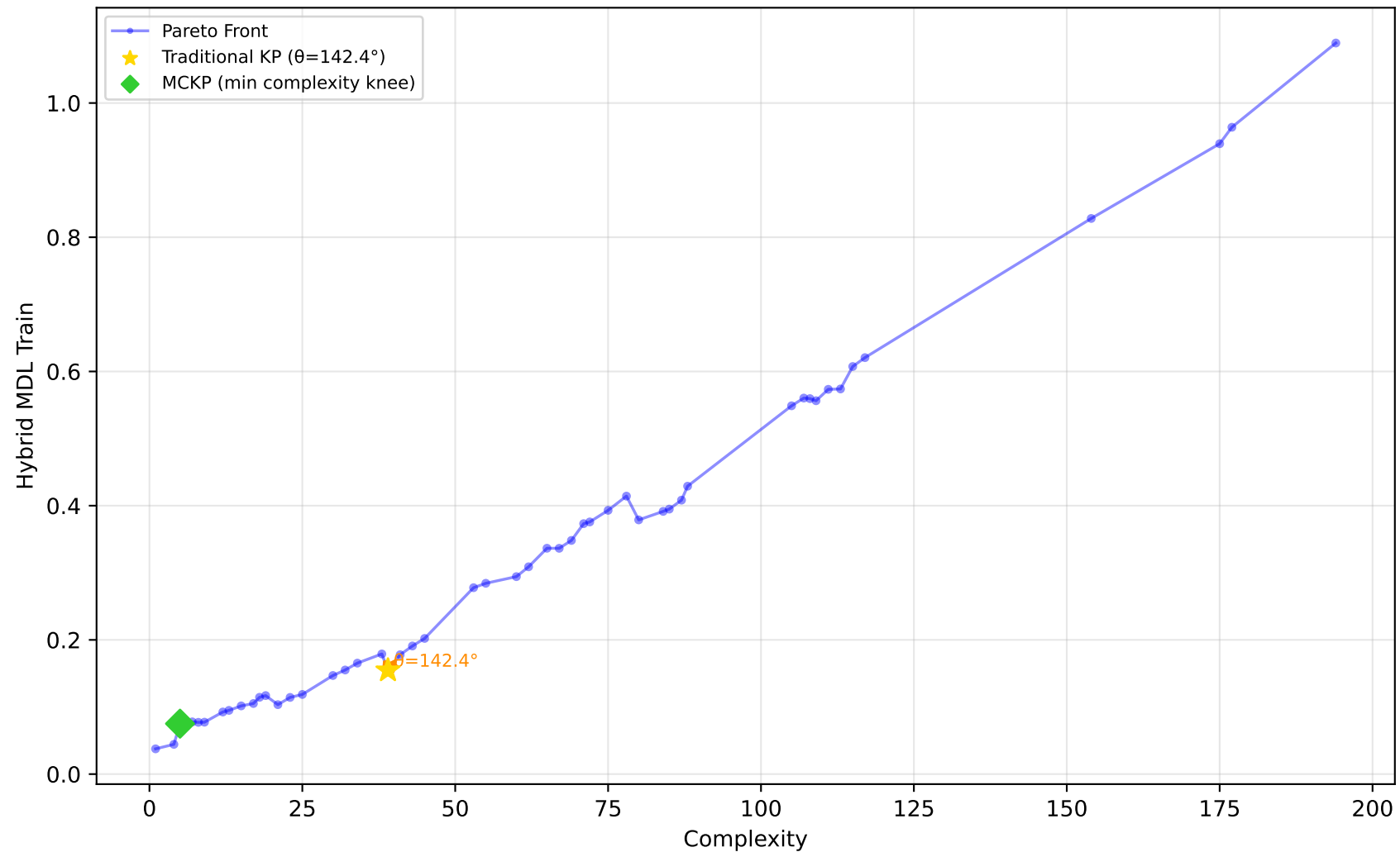
522_pm10 - Run 20 - SVP - Hybrid MDL Train \lambda_1=1.00, \lambda_2=0.00, \lambda_3=0.90 | Difficulty: 1.00 | Method: hmr
