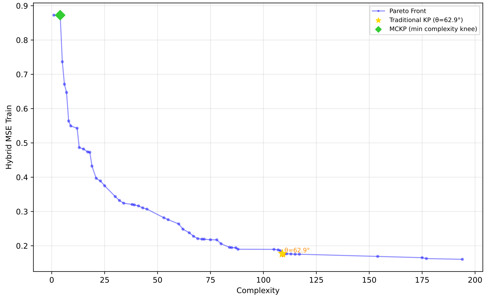
522_pm10 - Run 20 - SVP - Hybrid MSE Train \lambda_1=0.00, \lambda_2=0.10, \lambda_3=0.00 | Difficulty: 1.00 | Method: hmr
