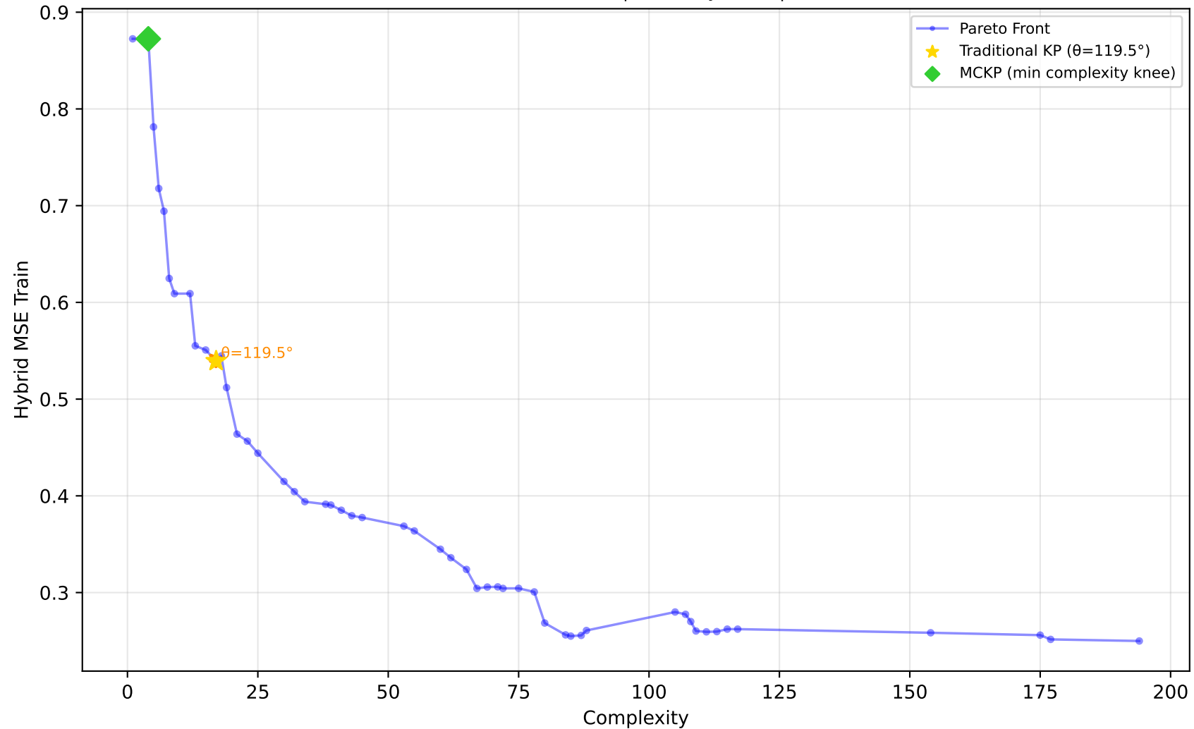
522_pm10 - Run 20 - SVP - Hybrid MSE Train \lambda_1=1.00, \lambda_2=0.00, \lambda_3=0.90 | Difficulty: 1.00 | Method: hmr
