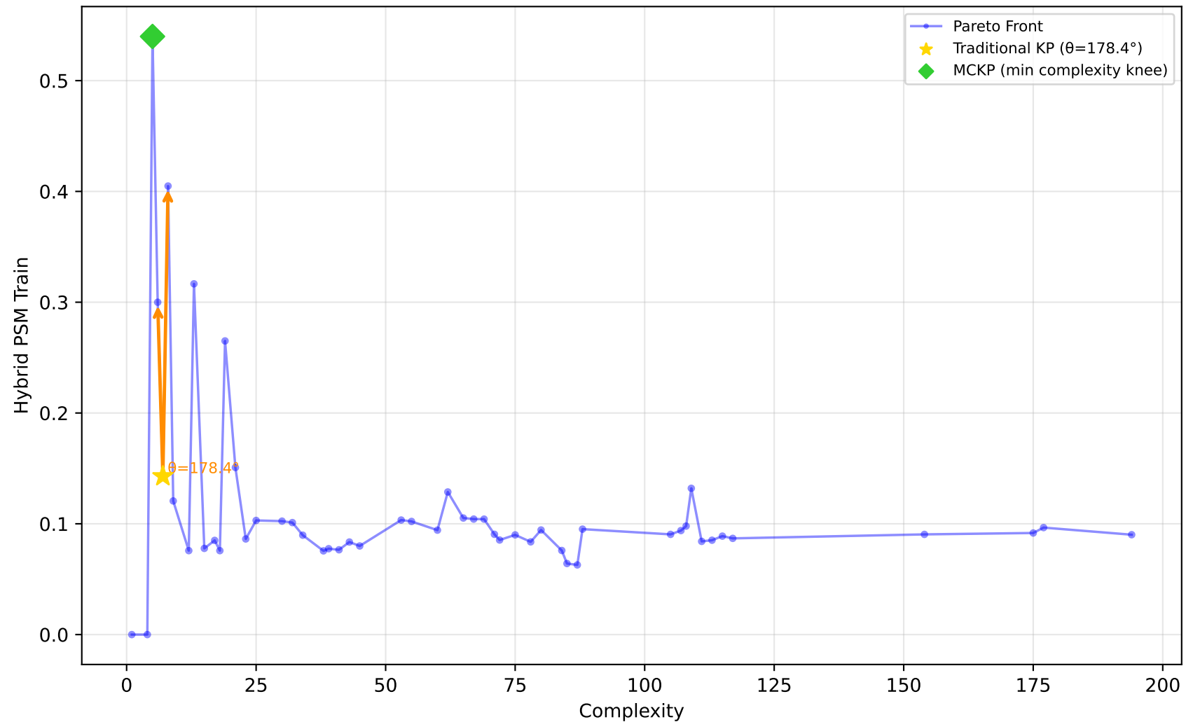
522_pm10 - Run 20 - SVP - Hybrid PSM Train \lambda_1=1.00, \lambda_2=0.00, \lambda_3=0.90 | Difficulty: 1.00 | Method: hmr
