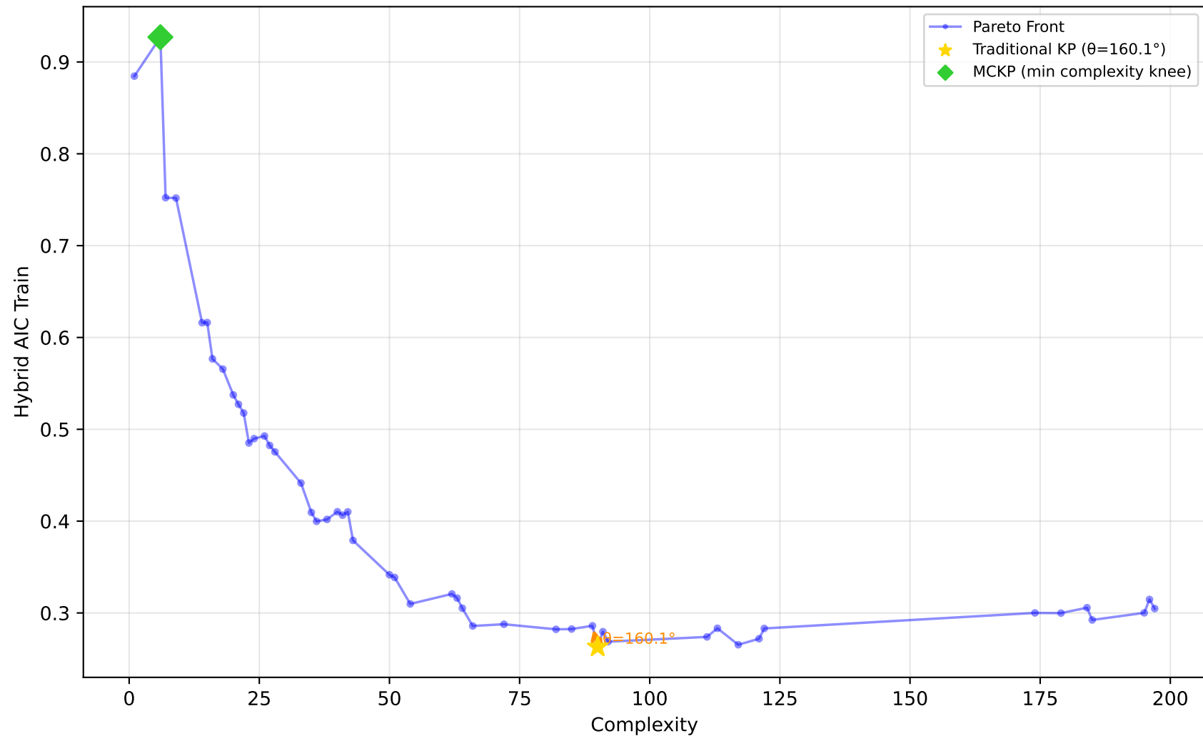
522_pm10 - Run 21 - MVP - Hybrid AIC Train \lambda_1=1.00, \lambda_2=0.00, \lambda_3=0.00 | Difficulty: 1.00 | Method: hmr
