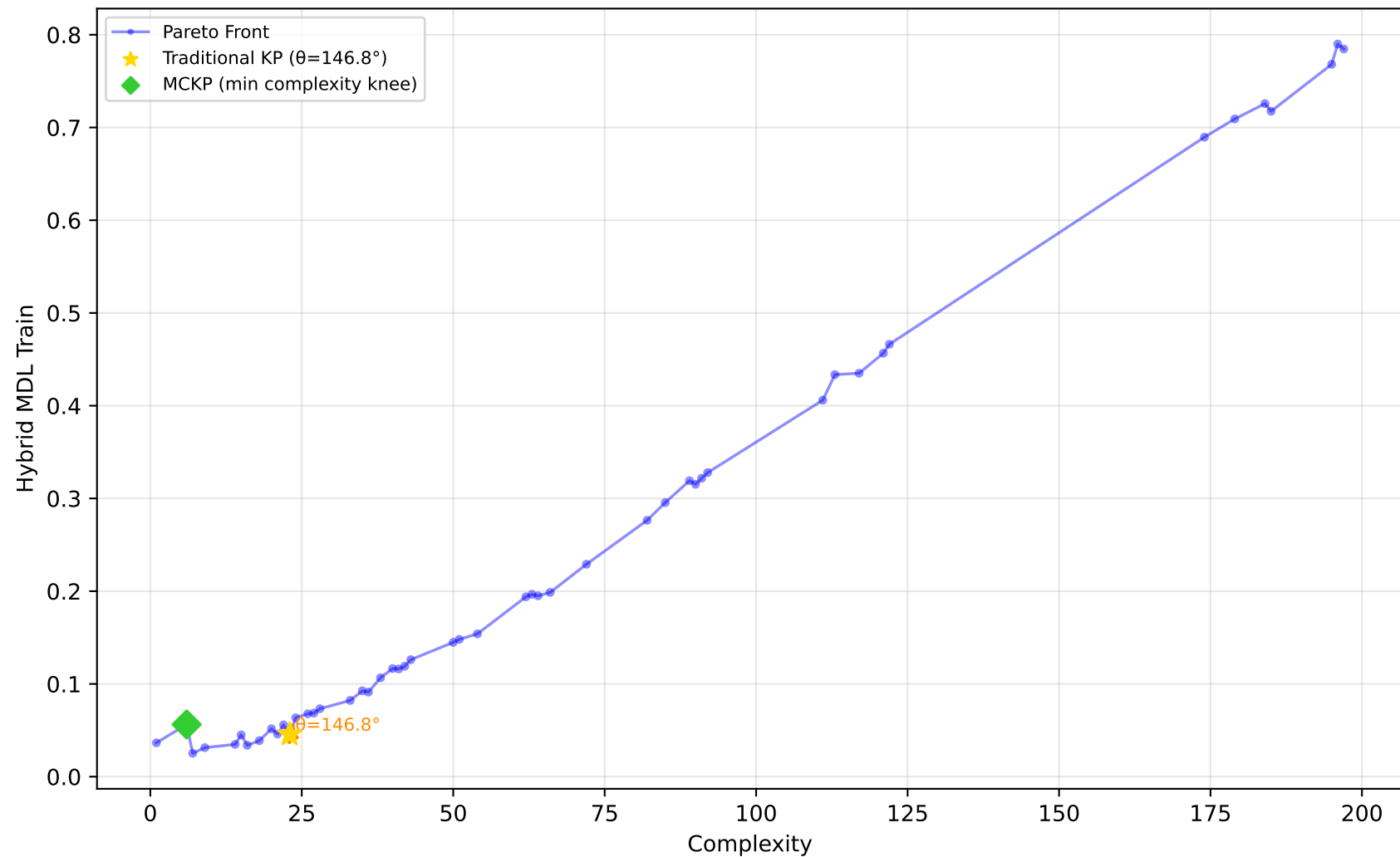
522_pm10 - Run 21 - MVP - Hybrid MDL Train \lambda_1=0.00, \lambda_2=0.90, \lambda_3=0.00 | Difficulty: 1.00 | Method: hmr
