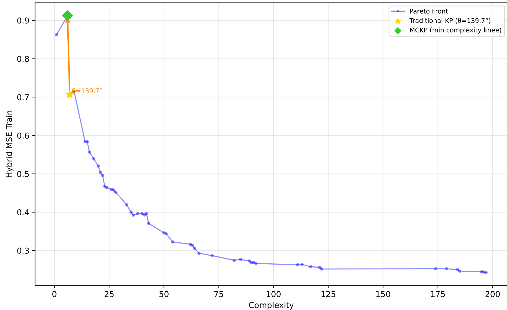
522_pm10 - Run 21 - MVP - Hybrid MSE Train \lambda_1=1.00, \lambda_2=0.00, \lambda_3=0.00 | Difficulty: 1.00 | Method: hmr
