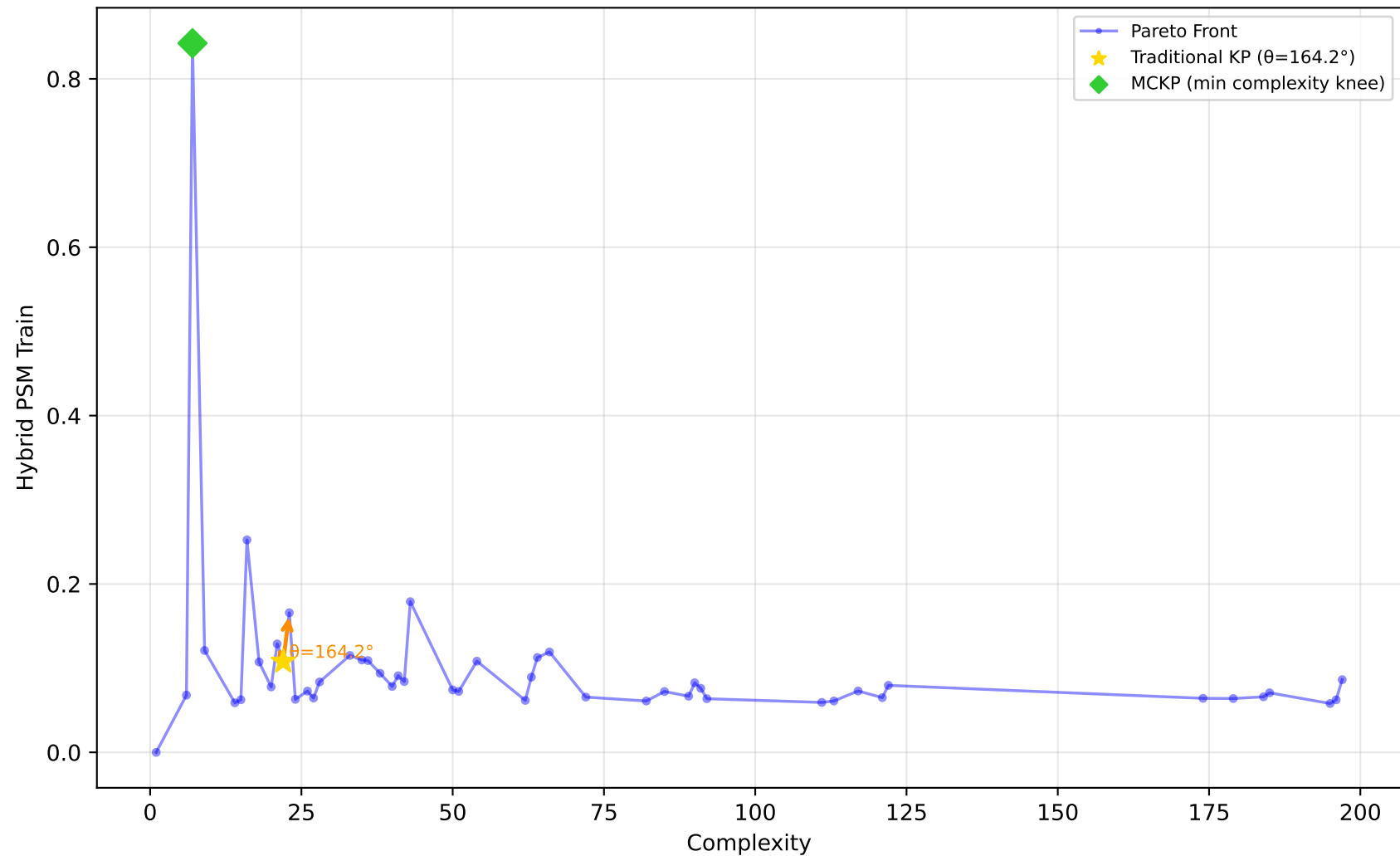
522_pm10 - Run 21 - MVP - Hybrid PSM Train \lambda_1=1.00, \lambda_2=0.00, \lambda_3=0.00 | Difficulty: 1.00 | Method: hmr
