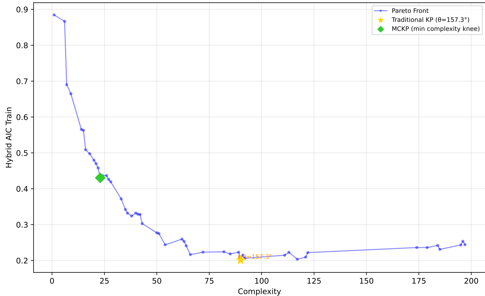
522_pm10 - Run 21 - SVP - Hybrid AIC Train \lambda_1=0.00, \lambda_2=0.10, \lambda_3=0.00 | Difficulty: 1.00 | Method: hmr
