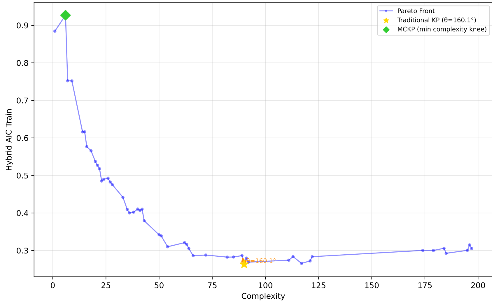
522_pm10 - Run 21 - SVP - Hybrid AIC Train \lambda_1=1.00, \lambda_2=0.00, \lambda_3=0.90 | Difficulty: 1.00 | Method: hmr
