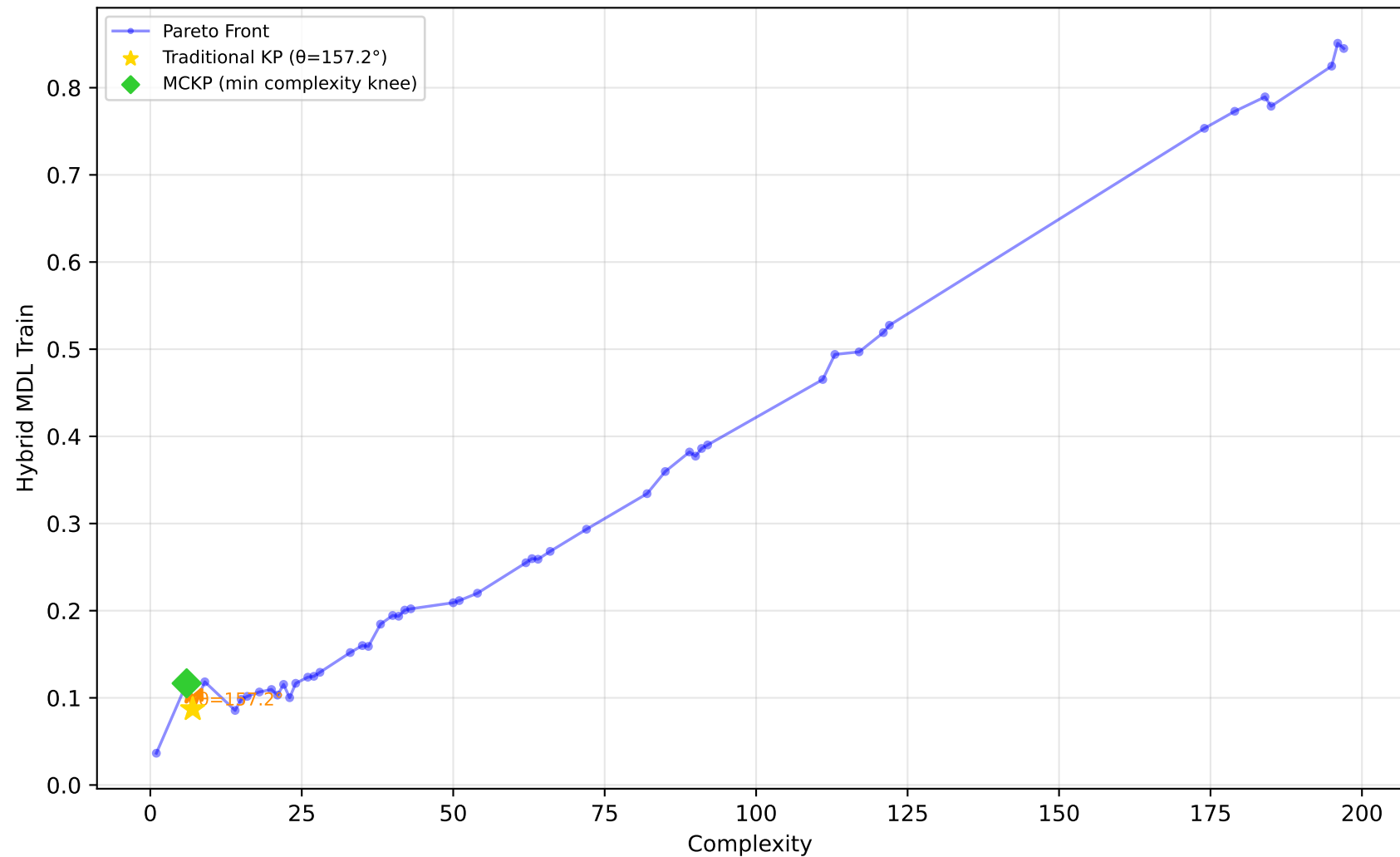
522_pm10 - Run 21 - SVP - Hybrid MDL Train \lambda_1=1.00, \lambda_2=0.00, \lambda_3=0.90 | Difficulty: 1.00 | Method: hmr
