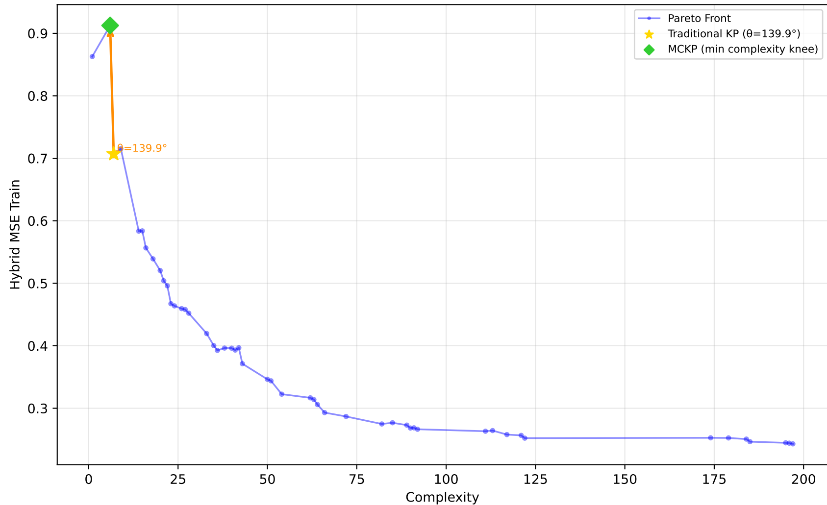
522_pm10 - Run 21 - SVP - Hybrid MSE Train \lambda_1=1.00, \lambda_2=0.00, \lambda_3=0.90 | Difficulty: 1.00 | Method: hmr
