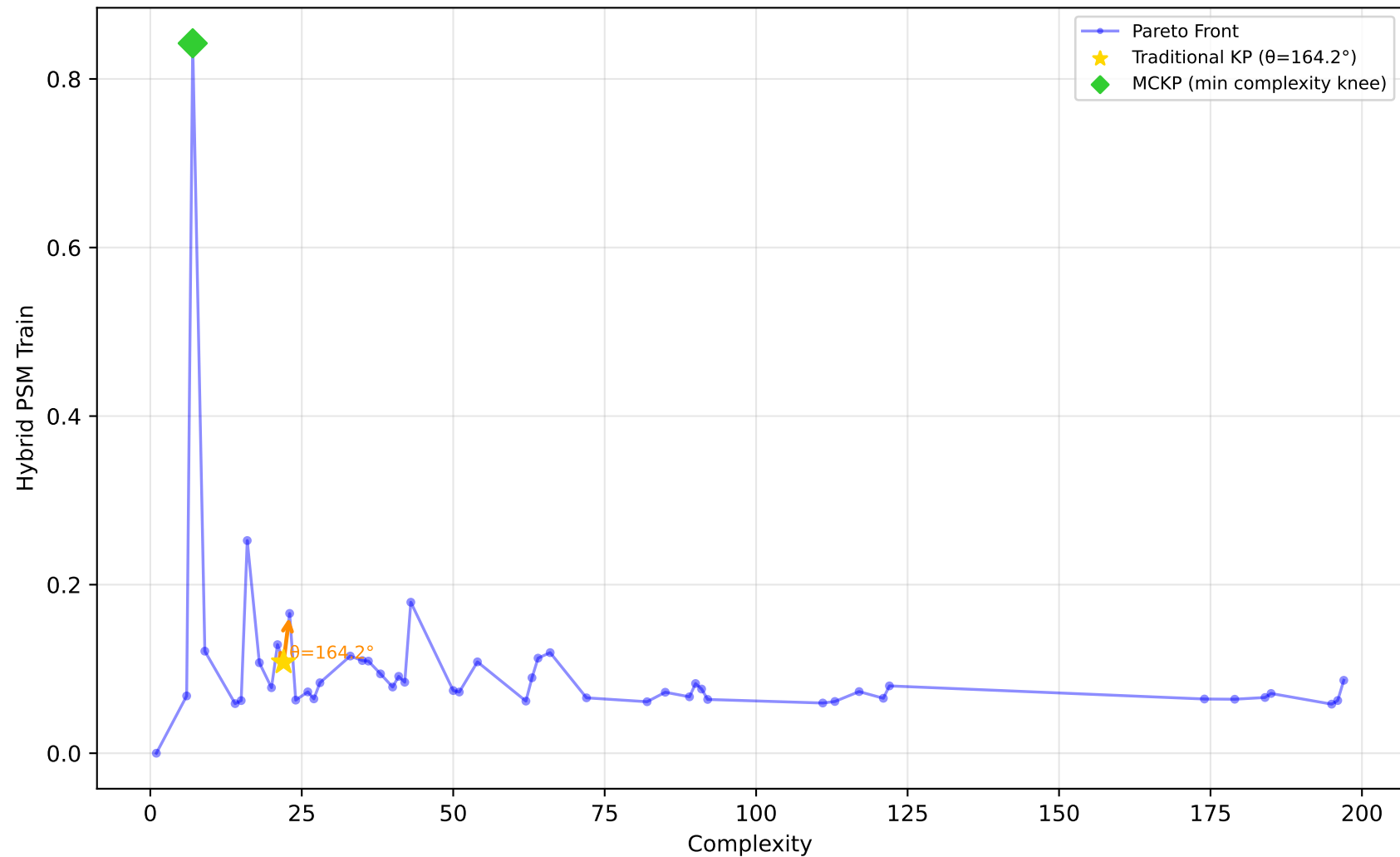
522_pm10 - Run 21 - SVP - Hybrid PSM Train \lambda_1=1.00, \lambda_2=0.00, \lambda_3=0.90 | Difficulty: 1.00 | Method: hmr
