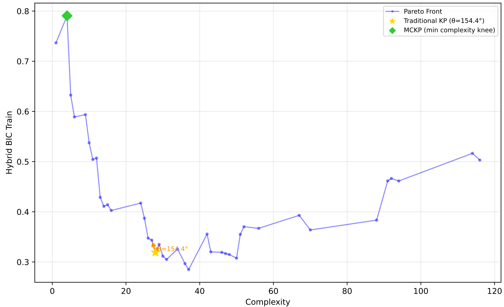
522_pm10 - Run 22 - MVP - Hybrid BIC Train \lambda_1=1.00, \lambda_2=0.00, \lambda_3=0.00 | Difficulty: 1.00 | Method: hmr
