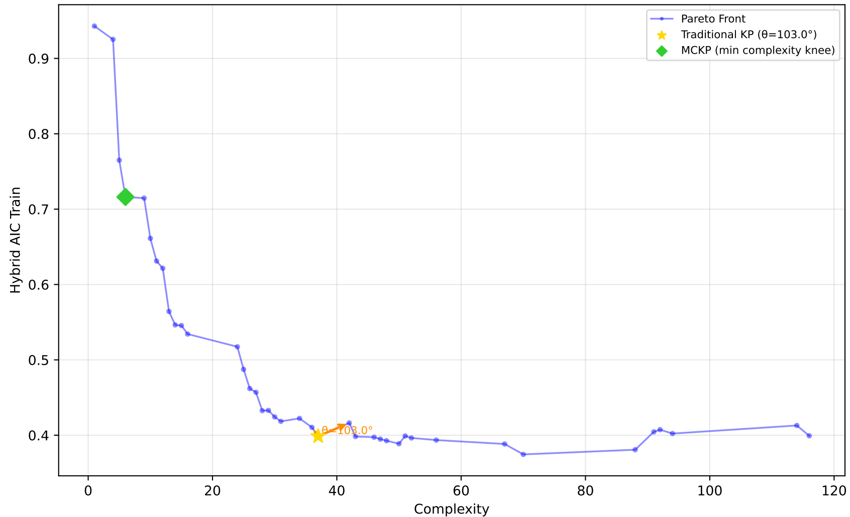
522_pm10 - Run 22 - SVP - Hybrid AIC Train \lambda_1=0.00, \lambda_2=0.10, \lambda_3=0.00 | Difficulty: 1.00 | Method: hmr
