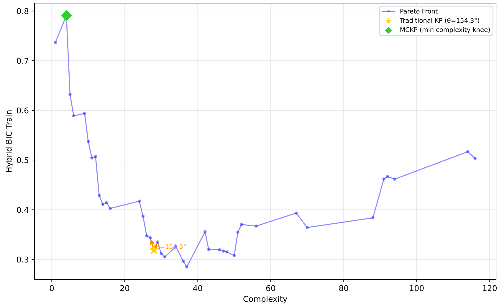
522_pm10 - Run 22 - SVP - Hybrid BIC Train \lambda_1=1.00, \lambda_2=0.00, \lambda_3=0.90 | Difficulty: 1.00 | Method: hmr
