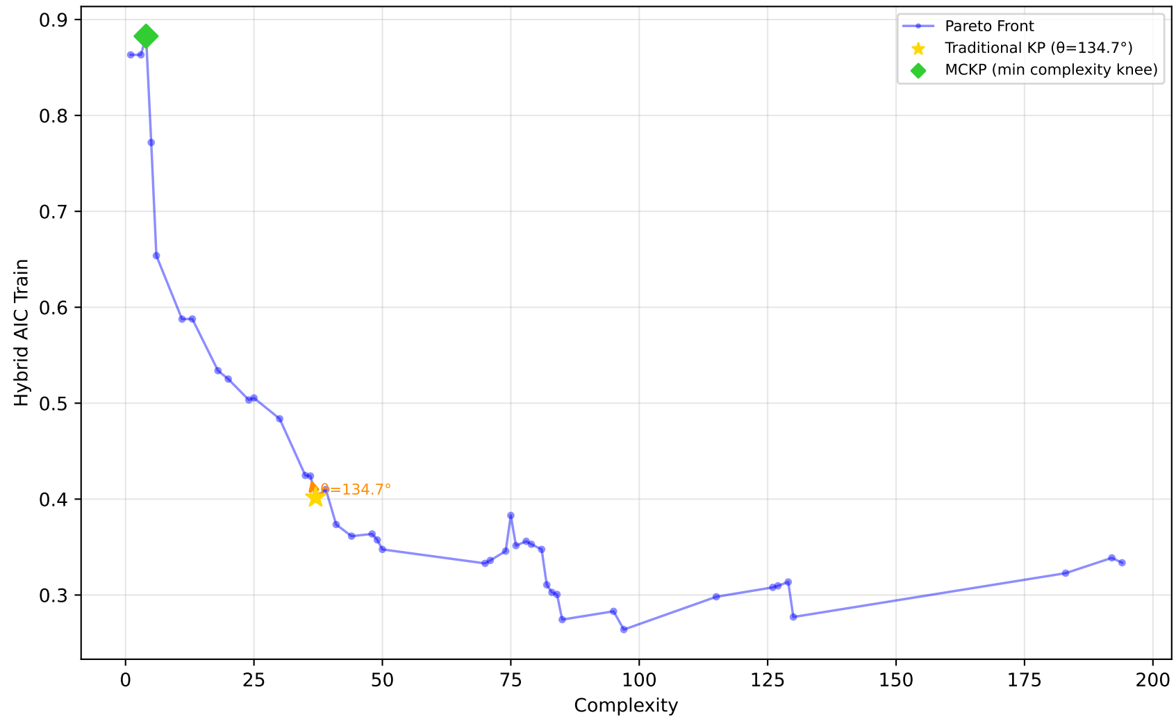
522_pm10 - Run 23 - MVP - Hybrid AIC Train \lambda_1=1.00, \lambda_2=0.00, \lambda_3=0.00 | Difficulty: 1.00 | Method: hmr
