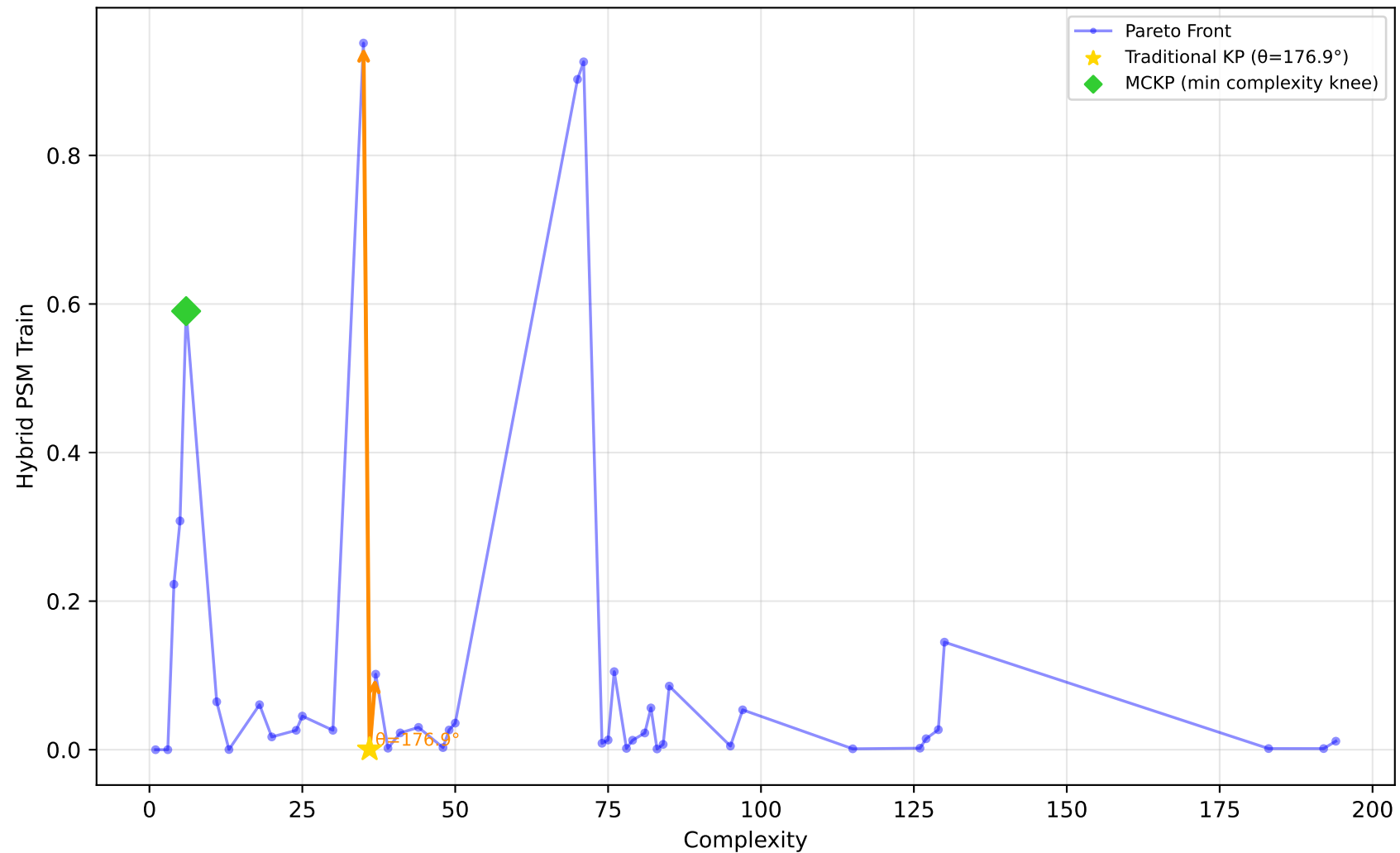
522_pm10 - Run 23 - MVP - Hybrid PSM Train \lambda_1=0.00, \lambda_2=0.90, \lambda_3=0.00 | Difficulty: 1.00 | Method: hmr
