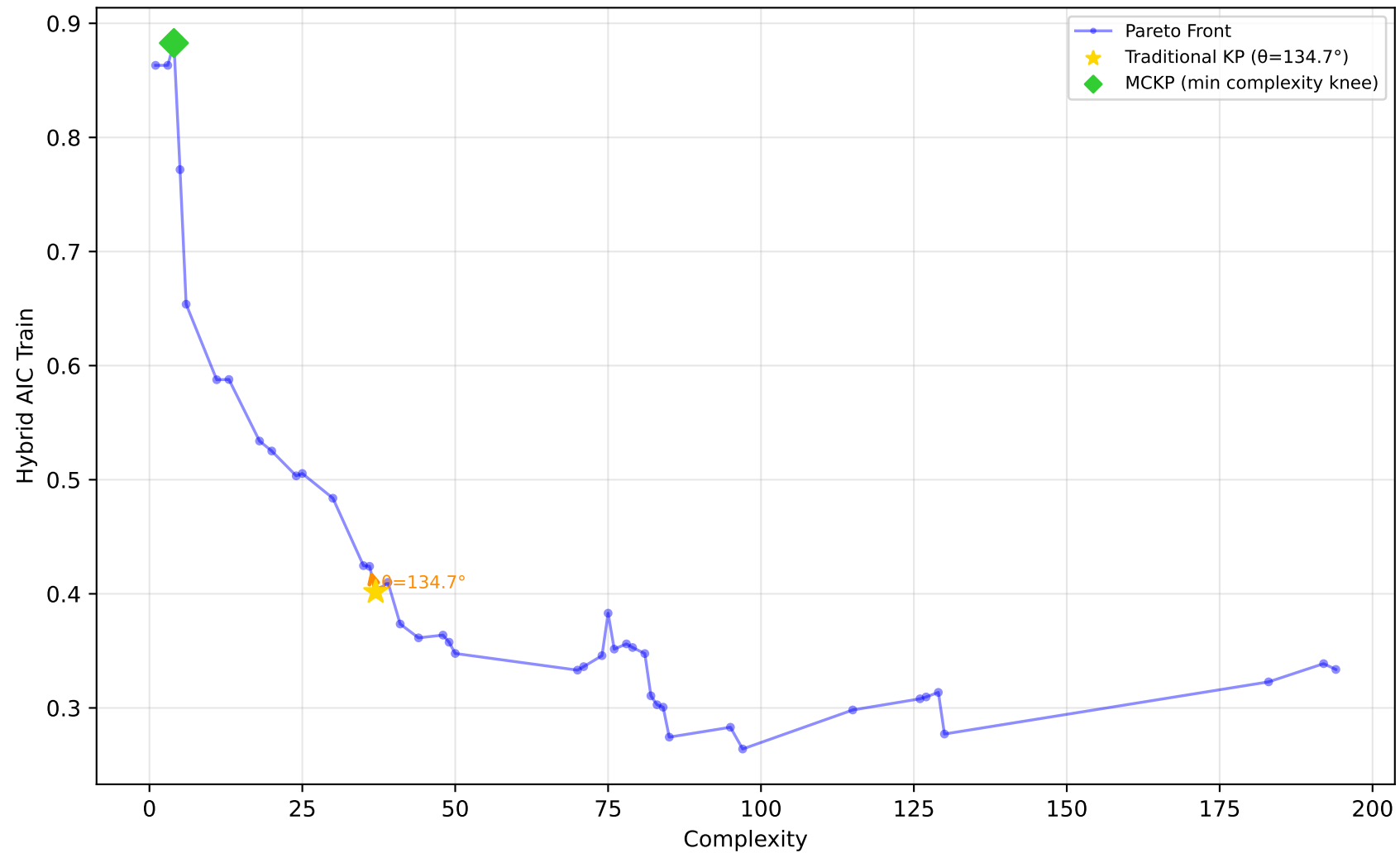
522_pm10 - Run 23 - SVP - Hybrid AIC Train \lambda_1=1.00, \lambda_2=0.00, \lambda_3=0.90 | Difficulty: 1.00 | Method: hmr
