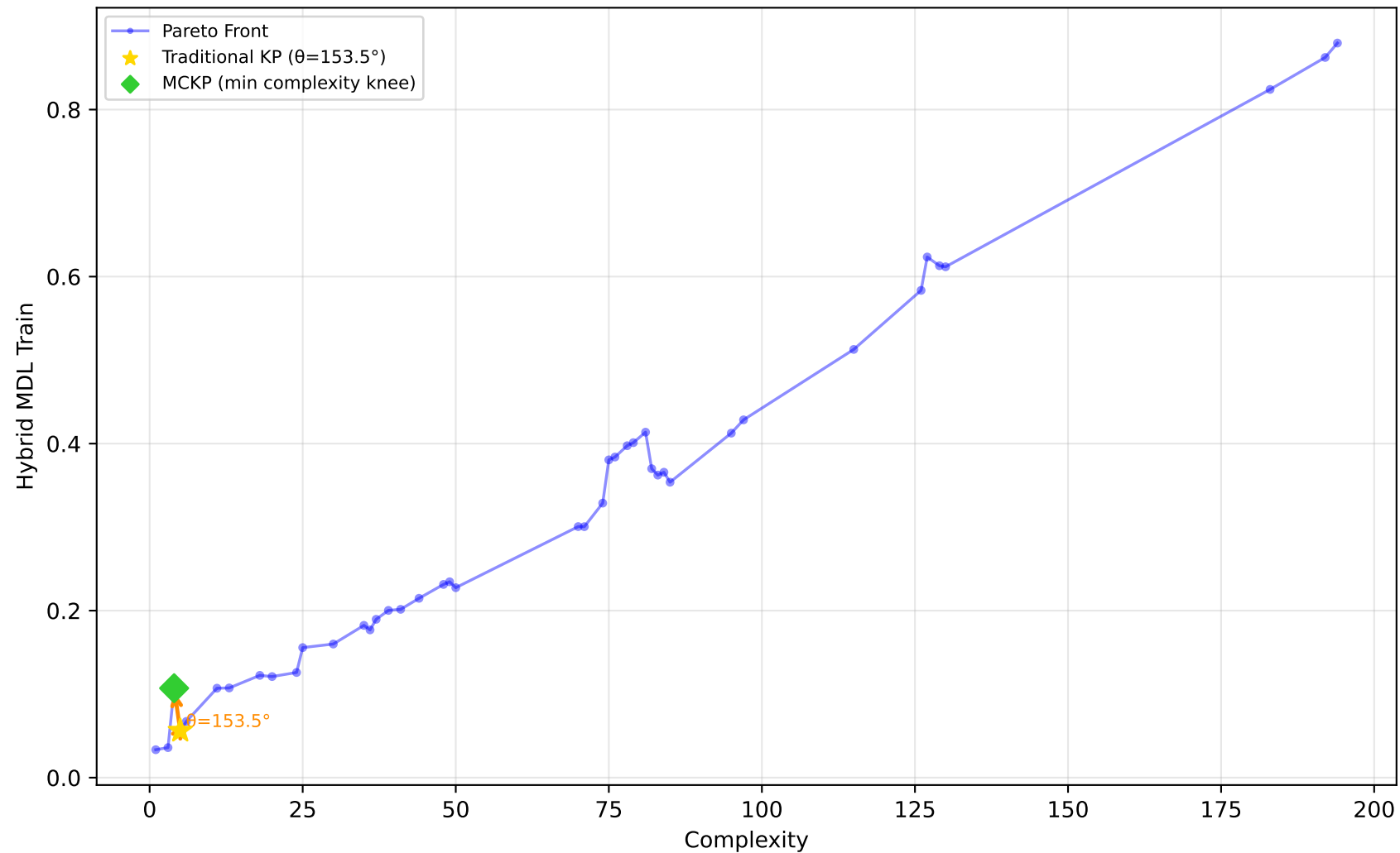
522_pm10 - Run 23 - SVP - Hybrid MDL Train \lambda_1=1.00, \lambda_2=0.00, \lambda_3=0.90 | Difficulty: 1.00 | Method: hmr
