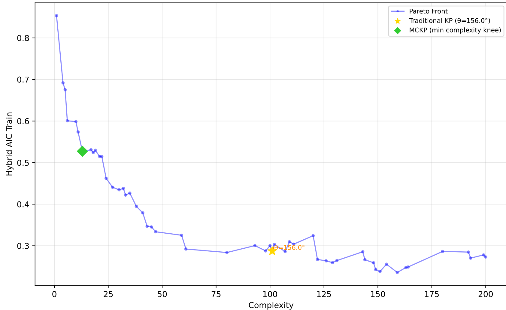
522_pm10 - Run 24 - MVP - Hybrid AIC Train \lambda_1=0.00, \lambda_2=0.90, \lambda_3=0.00 | Difficulty: 1.00 | Method: hmr
