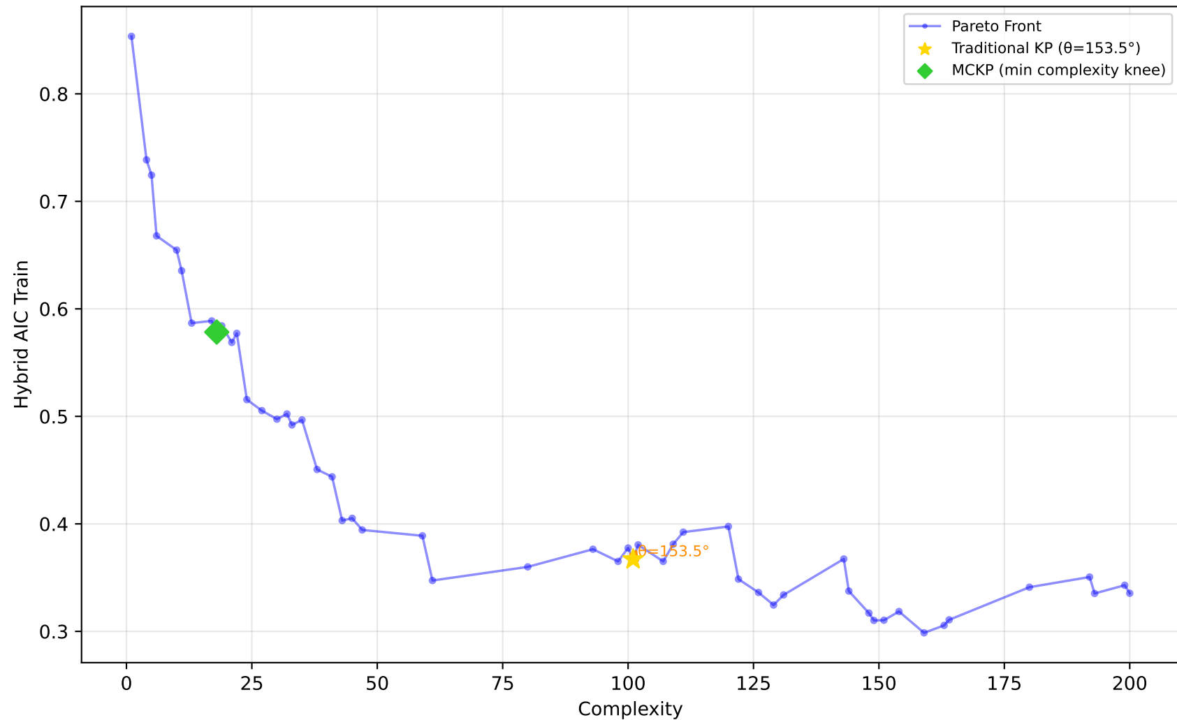
522_pm10 - Run 24 - MVP - Hybrid AIC Train \lambda_1=1.00, \lambda_2=0.00, \lambda_3=0.00 | Difficulty: 1.00 | Method: hmr
