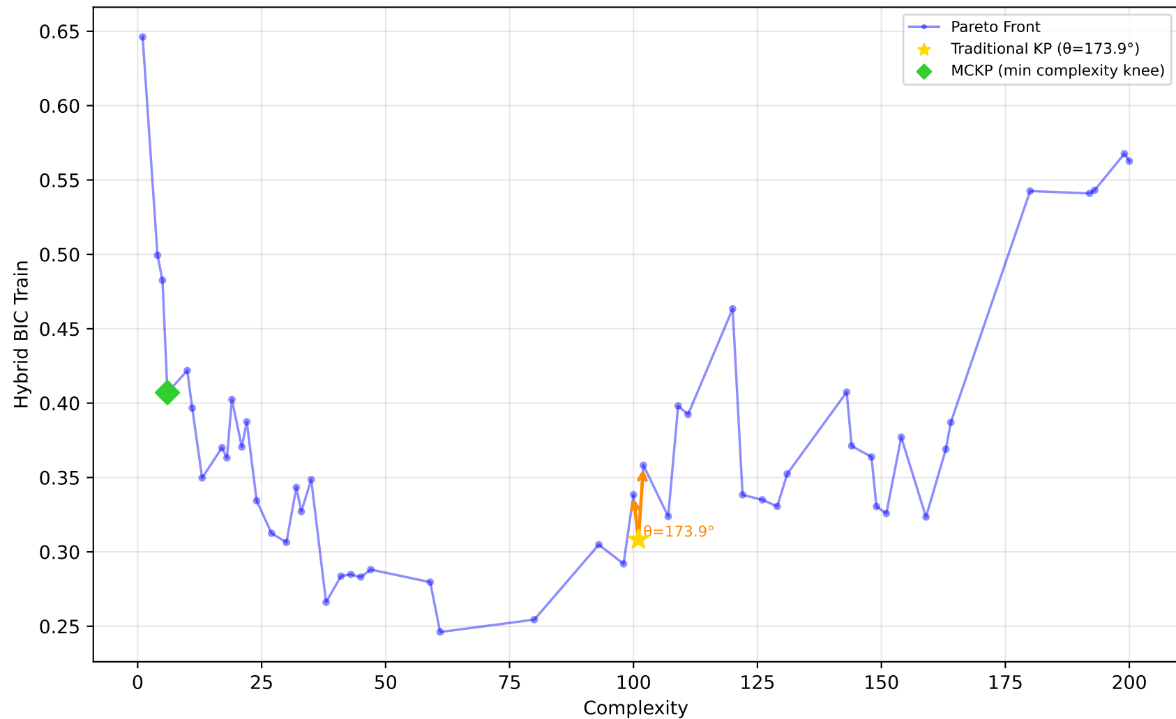
522_pm10 - Run 24 - MVP - Hybrid BIC Train \lambda_1=0.00, \lambda_2=0.90, \lambda_3=0.00 | Difficulty: 1.00 | Method: hmr
