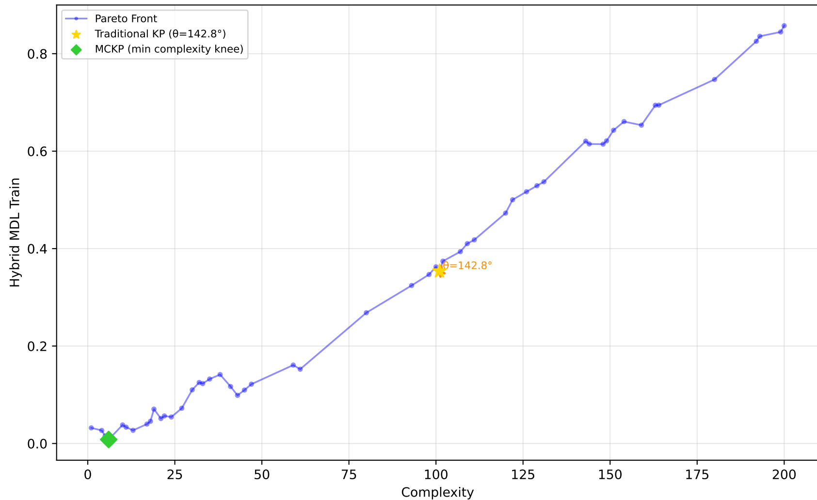
522_pm10 - Run 24 - MVP - Hybrid MDL Train \lambda_1=0.00, \lambda_2=0.90, \lambda_3=0.00 | Difficulty: 1.00 | Method: hmr
