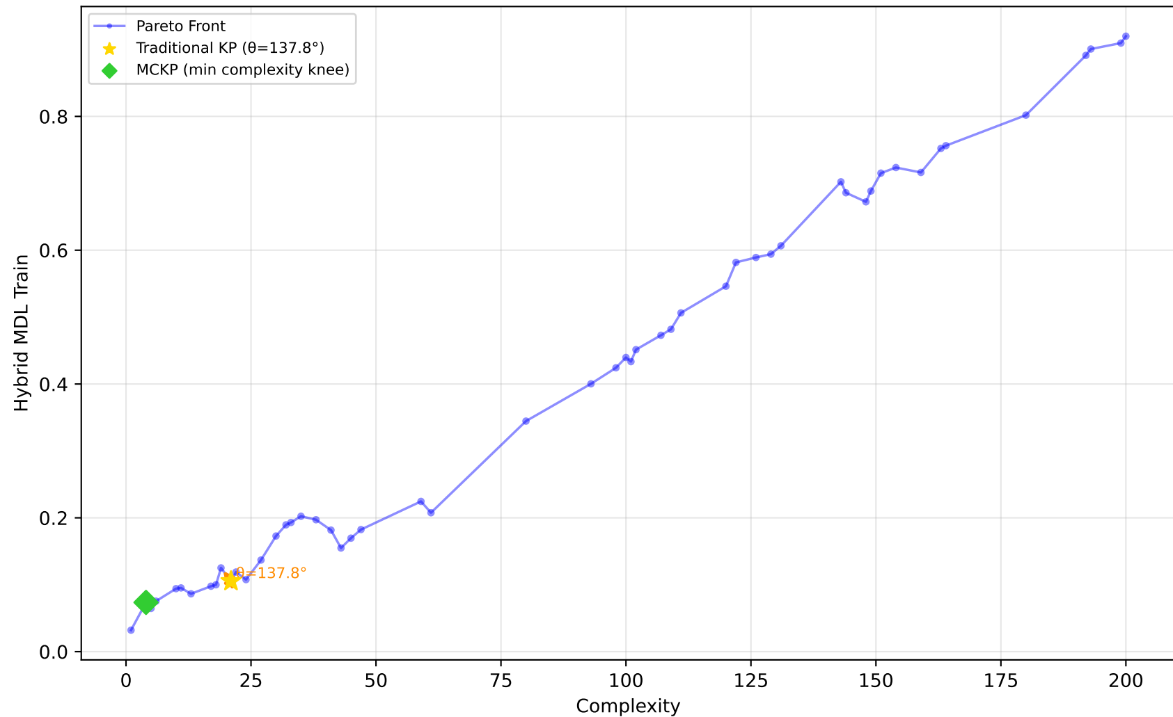
522_pm10 - Run 24 - MVP - Hybrid MDL Train \lambda_1=1.00, \lambda_2=0.00, \lambda_3=0.00 | Difficulty: 1.00 | Method: hmr
