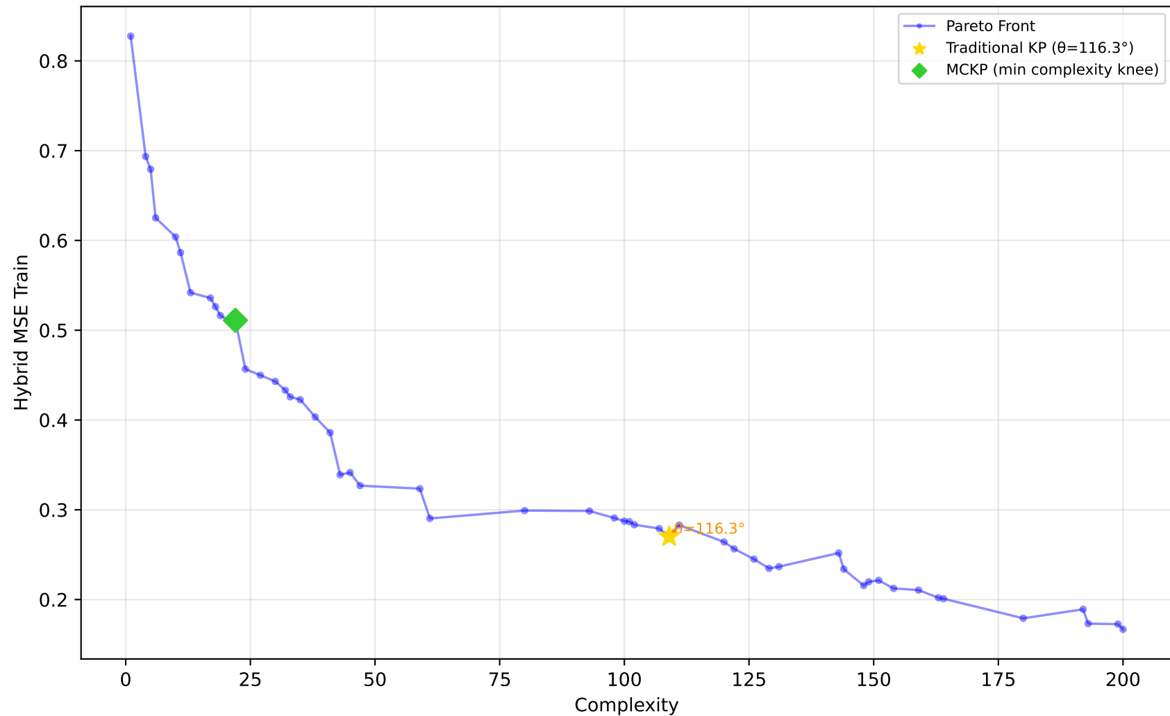
522_pm10 - Run 24 - MVP - Hybrid MSE Train \lambda_1=1.00, \lambda_2=0.00, \lambda_3=0.00 | Difficulty: 1.00 | Method: hmr
