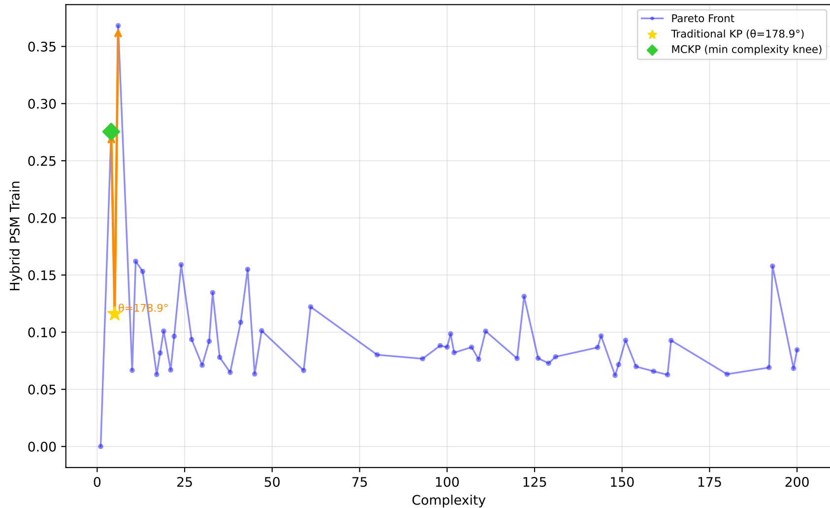
522_pm10 - Run 24 - MVP - Hybrid PSM Train \lambda_1=1.00, \lambda_2=0.00, \lambda_3=0.00 | Difficulty: 1.00 | Method: hmr
