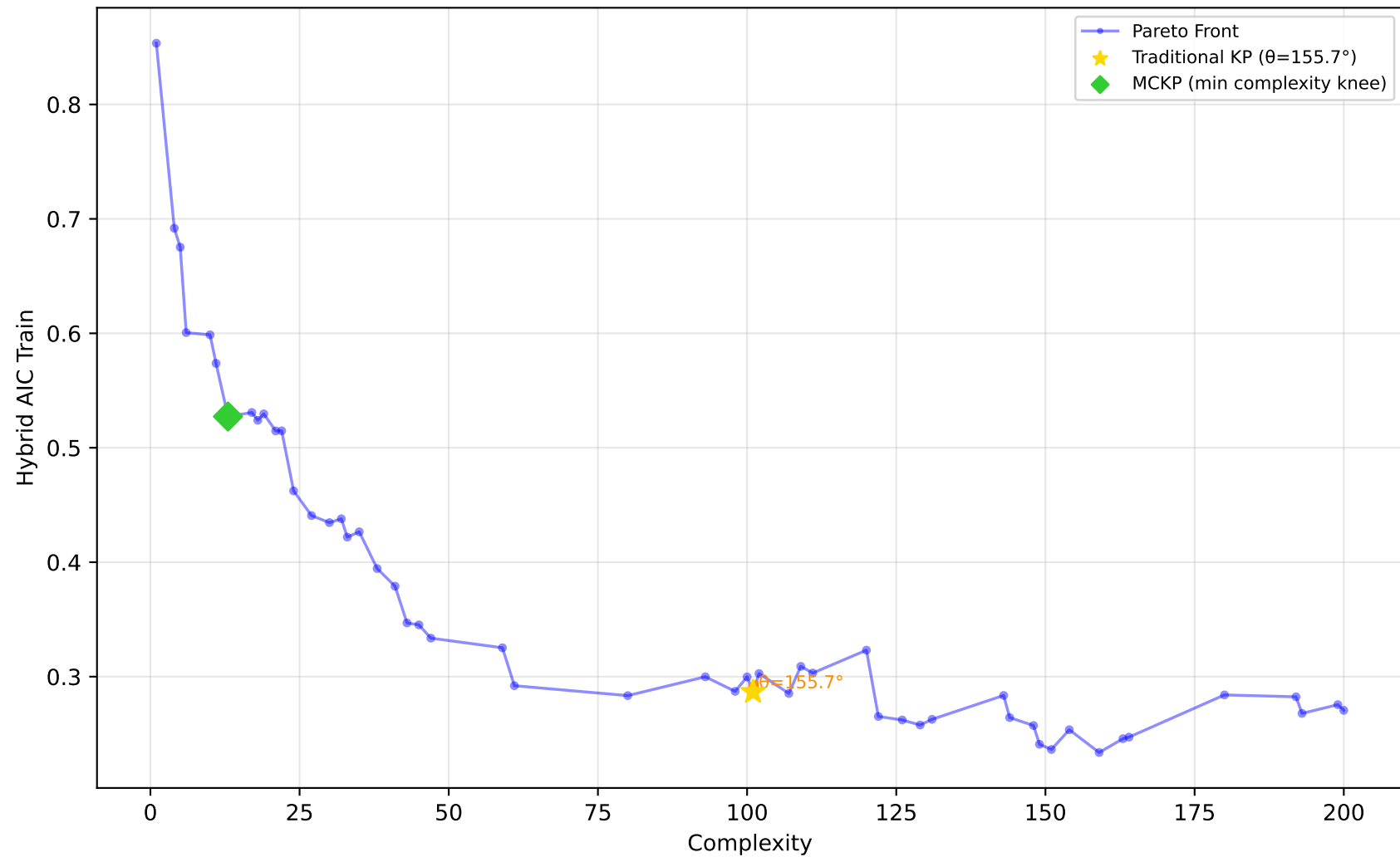
522_pm10 - Run 24 - SVP - Hybrid AIC Train \lambda_1=0.00, \lambda_2=0.10, \lambda_3=0.00 | Difficulty: 1.00 | Method: hmr
