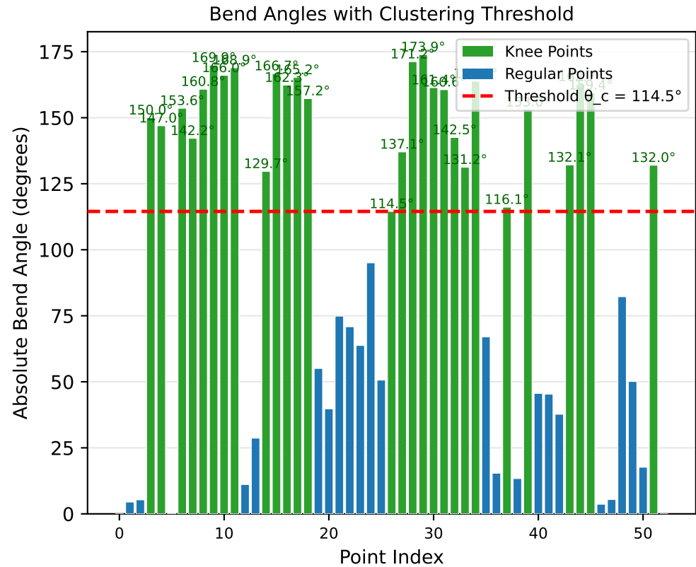
522_pm10 - Run 24 - SVP - Hybrid BIC Train - Clustering Threshold \lambda_1=0.00, \lambda_2=0.10, \lambda_3=0.00 | Difficulty: 1.00
