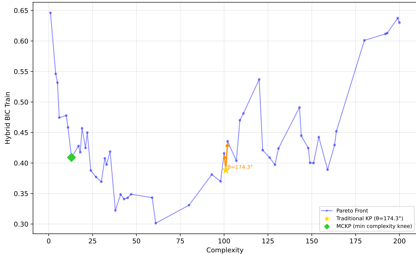
522_pm10 - Run 24 - SVP - Hybrid BIC Train \lambda_1=1.00, \lambda_2=0.00, \lambda_3=0.90 | Difficulty: 1.00 | Method: hmr
