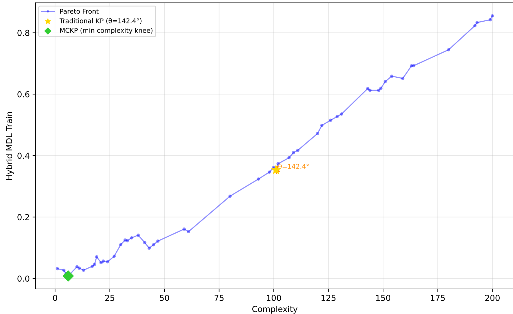
522_pm10 - Run 24 - SVP - Hybrid MDL Train \lambda_1=0.00, \lambda_2=0.10, \lambda_3=0.00 | Difficulty: 1.00 | Method: hmr
