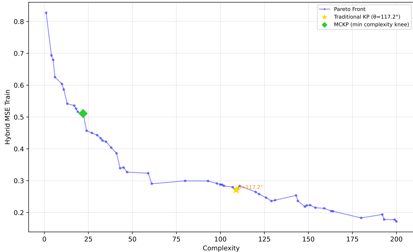
522_pm10 - Run 24 - SVP - Hybrid MSE Train \lambda_1=1.00, \lambda_2=0.00, \lambda_3=0.90 | Difficulty: 1.00 | Method: hmr
