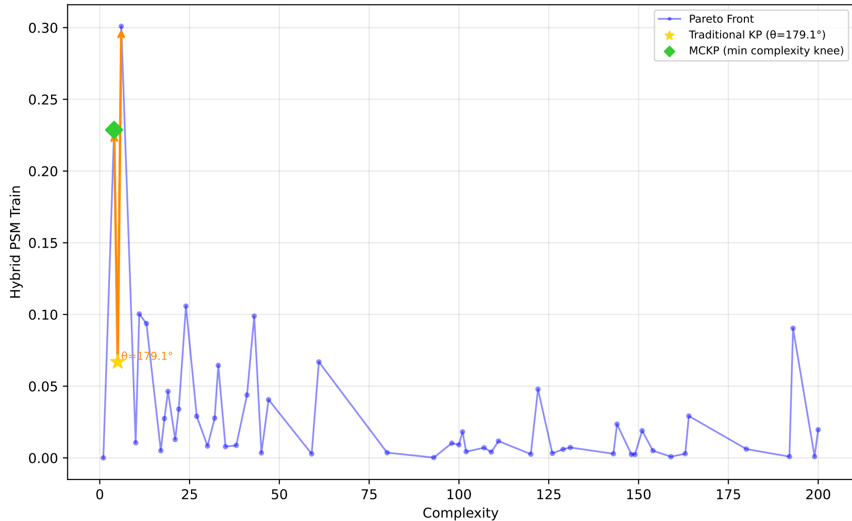
522_pm10 - Run 24 - SVP - Hybrid PSM Train \lambda_1=0.00, \lambda_2=0.10, \lambda_3=0.00 | Difficulty: 1.00 | Method: hmr
