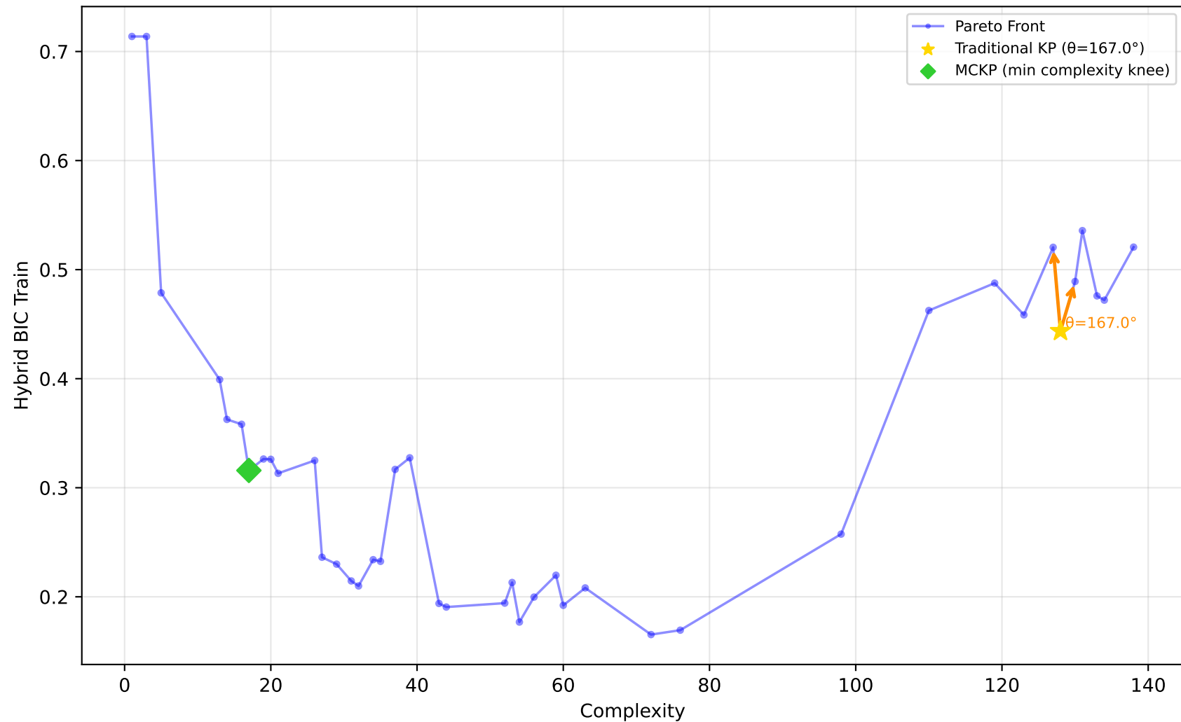
522_pm10 - Run 25 - MVP - Hybrid BIC Train \lambda_1=0.00, \lambda_2=0.90, \lambda_3=0.00 | Difficulty: 0.97 | Method: hmr
