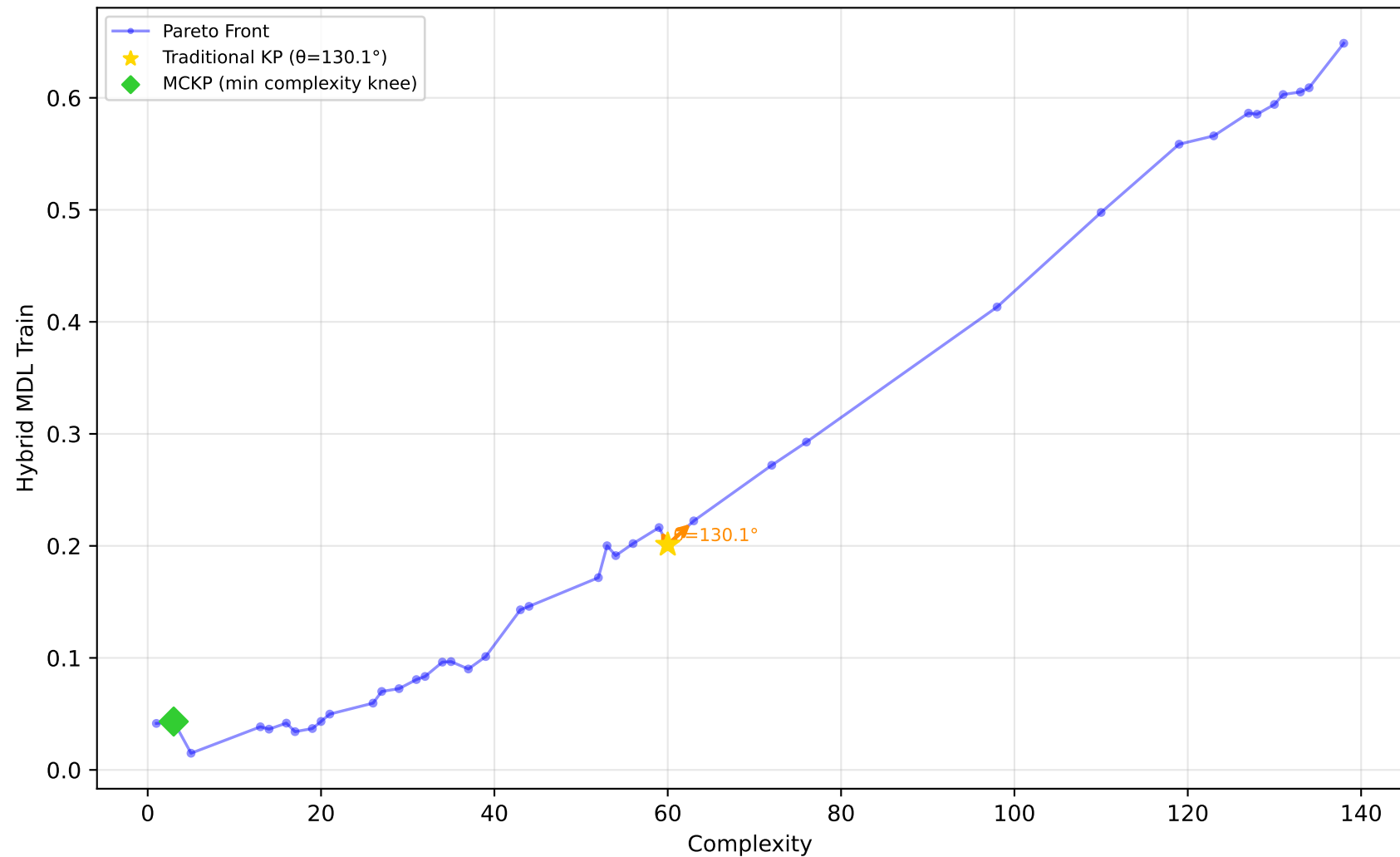
522_pm10 - Run 25 - MVP - Hybrid MDL Train \lambda_1=0.00, \lambda_2=0.90, \lambda_3=0.00 | Difficulty: 0.97 | Method: hmr
